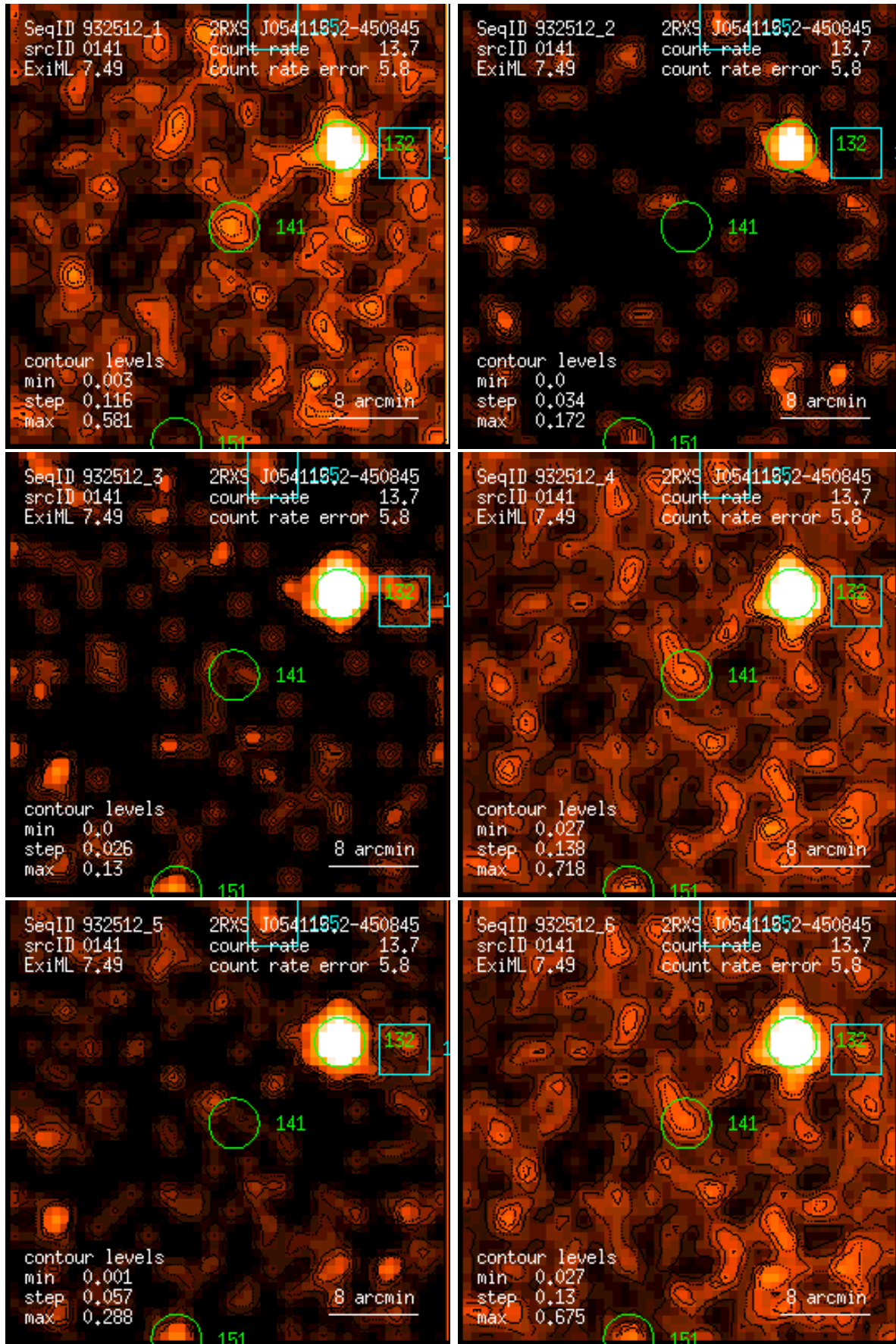
Figure 141: RASS 932512: detection 0141: band rate images, Gaussian filter: (1) PSPC channels 11 – 41, (2) 52 – 90, (3) 91 – 201, (4) 11 – 235, (5) 52 – 201, (6) 11 – 201. Broad band rates in counts/ks. Band rate contour levels in counts/ks/arcmin 2 .
