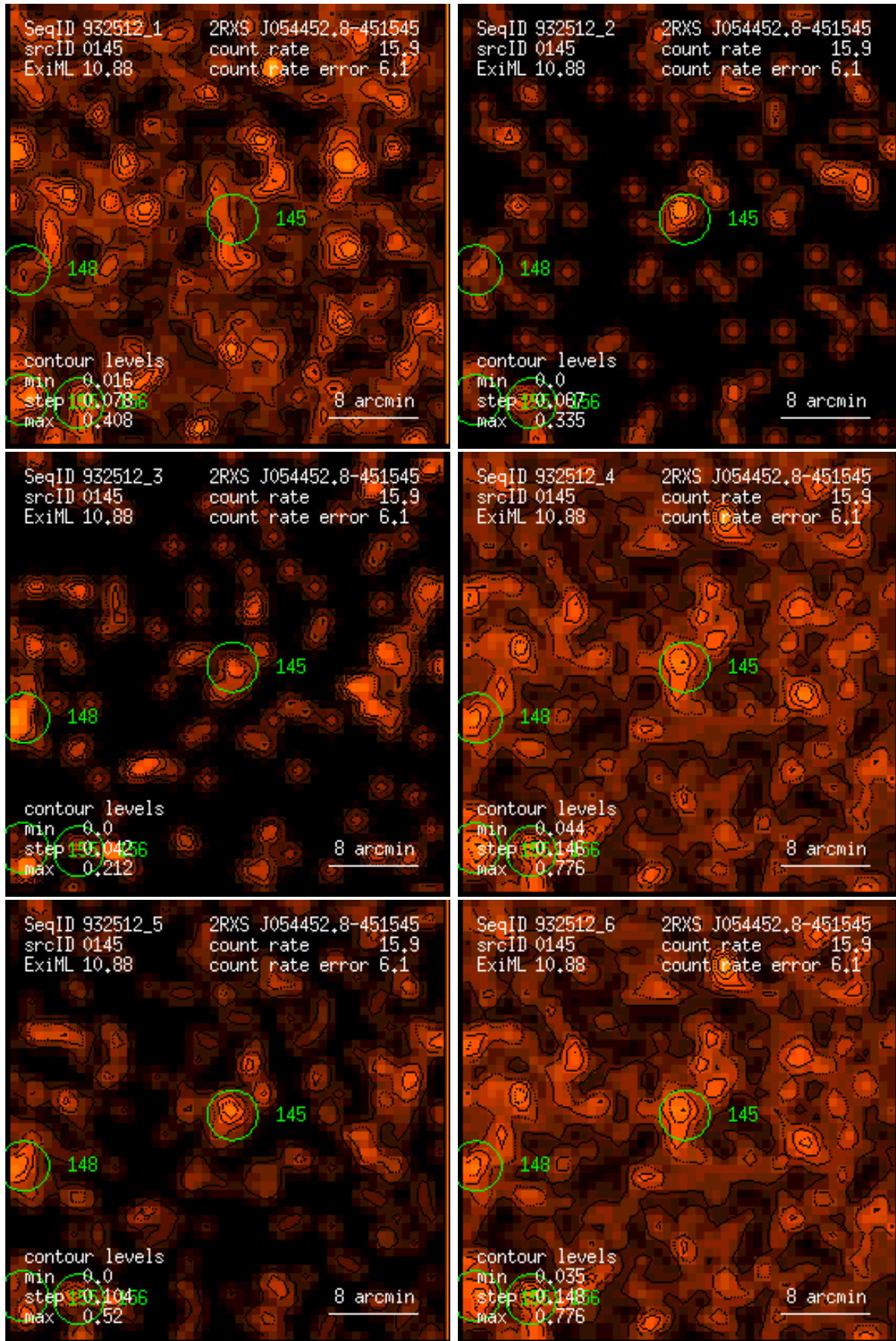
Figure 145: RASS 932512: detection 0145: band rate images, Gaussian filter: (1) PSPC channels 11 – 41, (2) 52 – 90, (3) 91 – 201, (4) 11 – 235, (5) 52 – 201, (6) 11 – 201. Broad band rates in counts/ks. Band rate contour levels in counts/ks/arcmin 2 .
