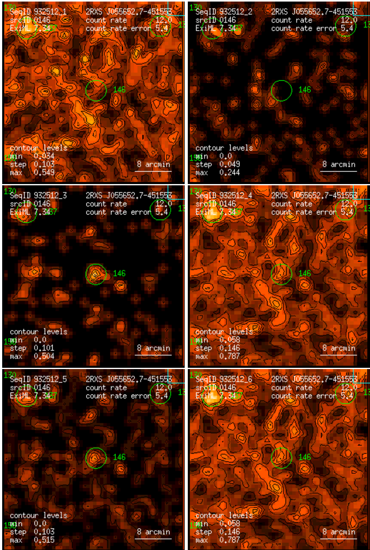
Figure 146: RASS 932512: detection 0146: band rate images, Gaussian filter: (1) PSPC channels 11 – 41, (2) 52 – 90, (3) 91 – 201, (4) 11 – 235, (5) 52 – 201, (6) 11 – 201. Broad band rates in counts/ks. Band rate contour levels in counts/ks/arcmin 2 .
