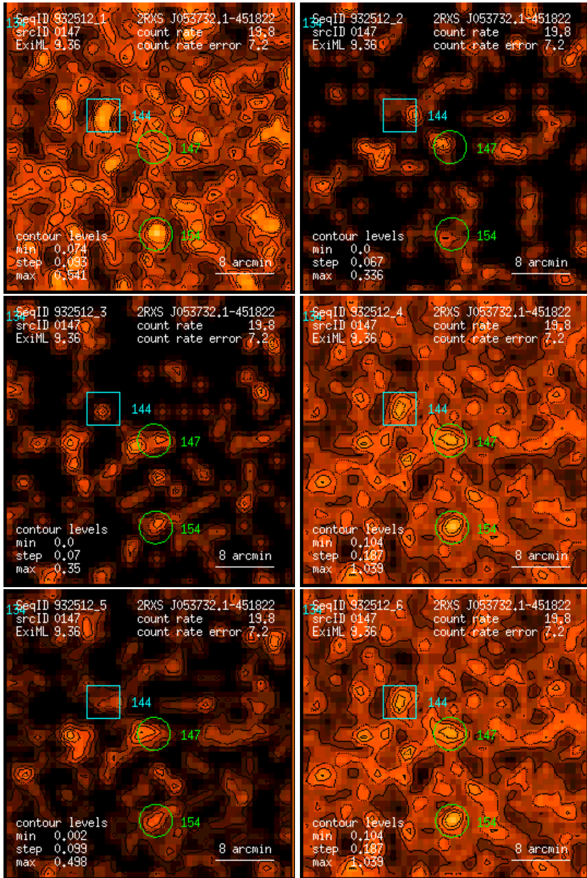
Figure 147: RASS 932512: detection 0147: band rate images, Gaussian filter: (1) PSPC channels 11 – 41, (2) 52 – 90, (3) 91 – 201, (4) 11 – 235, (5) 52 – 201, (6) 11 – 201. Broad band rates in counts/ks. Band rate contour levels in counts/ks/arcmin 2 .
