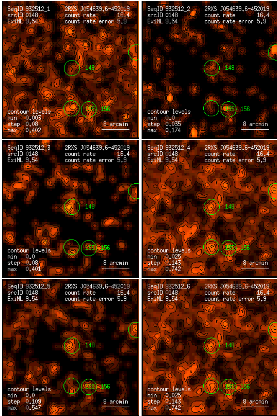
Figure 148: RASS 932512: detection 0148: band rate images, Gaussian filter: (1) PSPC channels 11 – 41, (2) 52 – 90, (3) 91 – 201, (4) 11 – 235, (5) 52 – 201, (6) 11 – 201. Broad band rates in counts/ks. Band rate contour levels in counts/ks/arcmin 2 .
