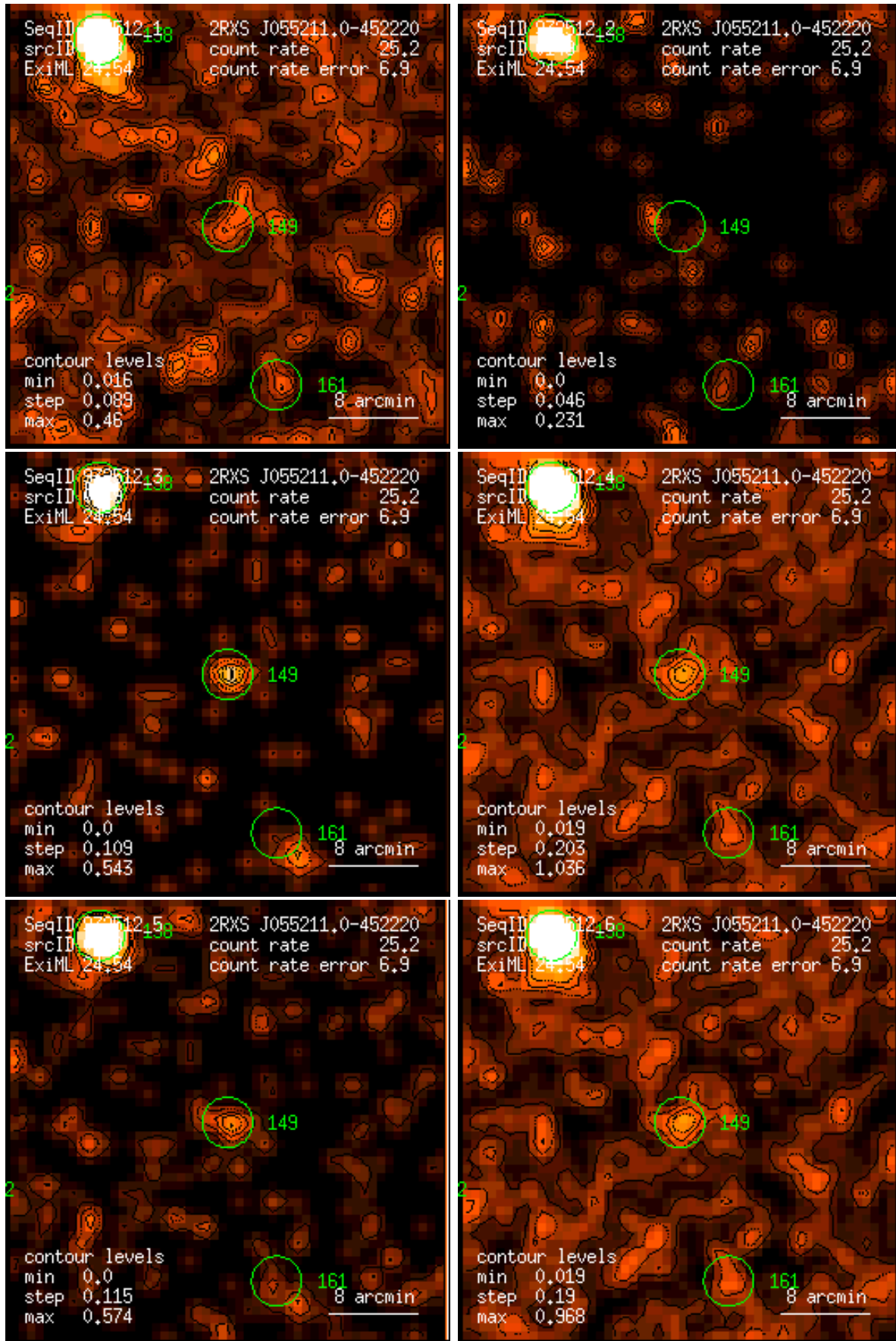
Figure 149: RASS 932512: detection 0149: band rate images, Gaussian filter: (1) PSPC channels 11 – 41, (2) 52 – 90, (3) 91 – 201, (4) 11 – 235, (5) 52 – 201, (6) 11 – 201. Broad band rates in counts/ks. Band rate contour levels in counts/ks/arcmin 2 .
