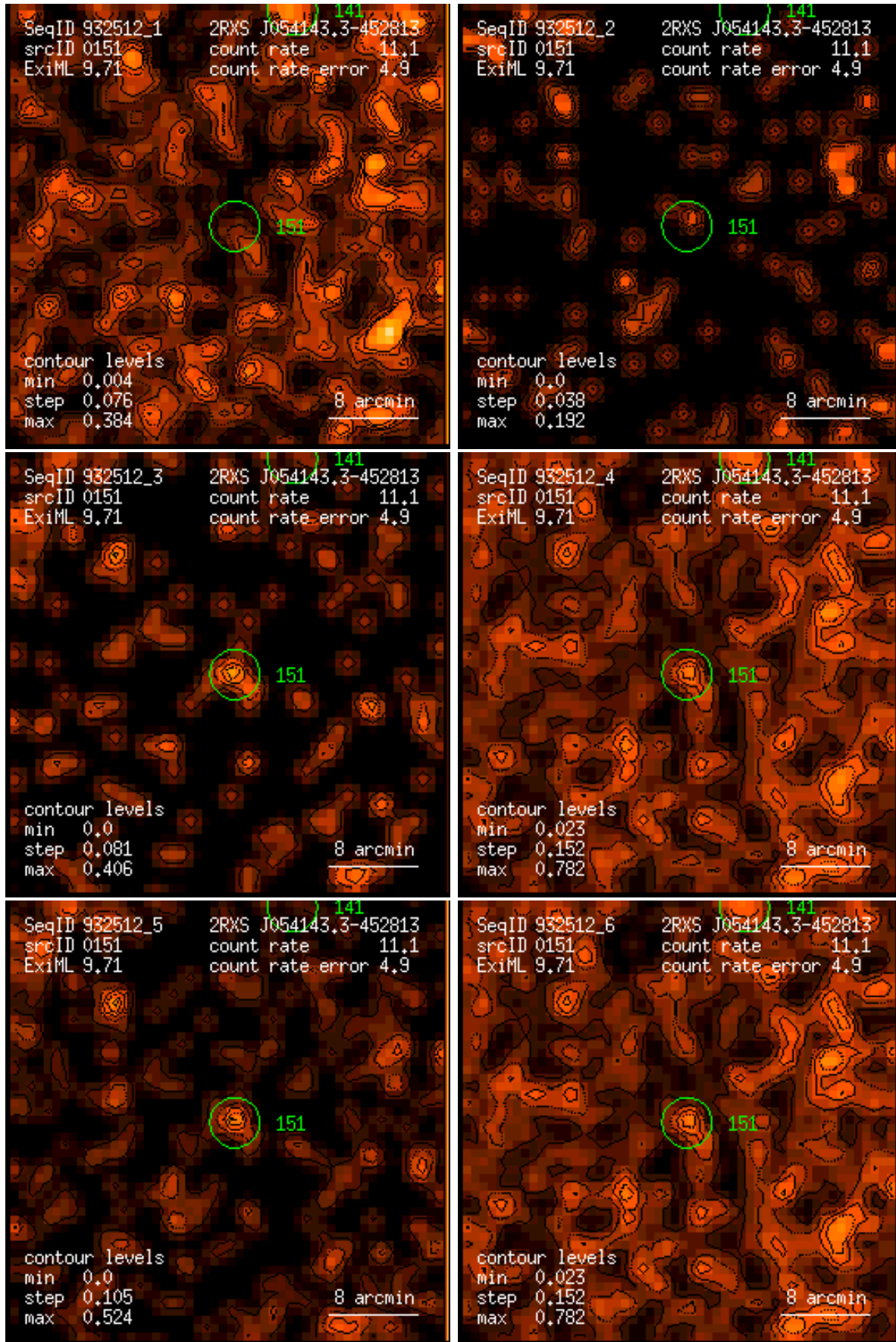
Figure 151: RASS 932512: detection 0151: band rate images, Gaussian filter: (1) PSPC channels 11 – 41, (2) 52 – 90, (3) 91 – 201, (4) 11 – 235, (5) 52 – 201, (6) 11 – 201. Broad band rates in counts/ks. Band rate contour levels in counts/ks/arcmin 2 .
