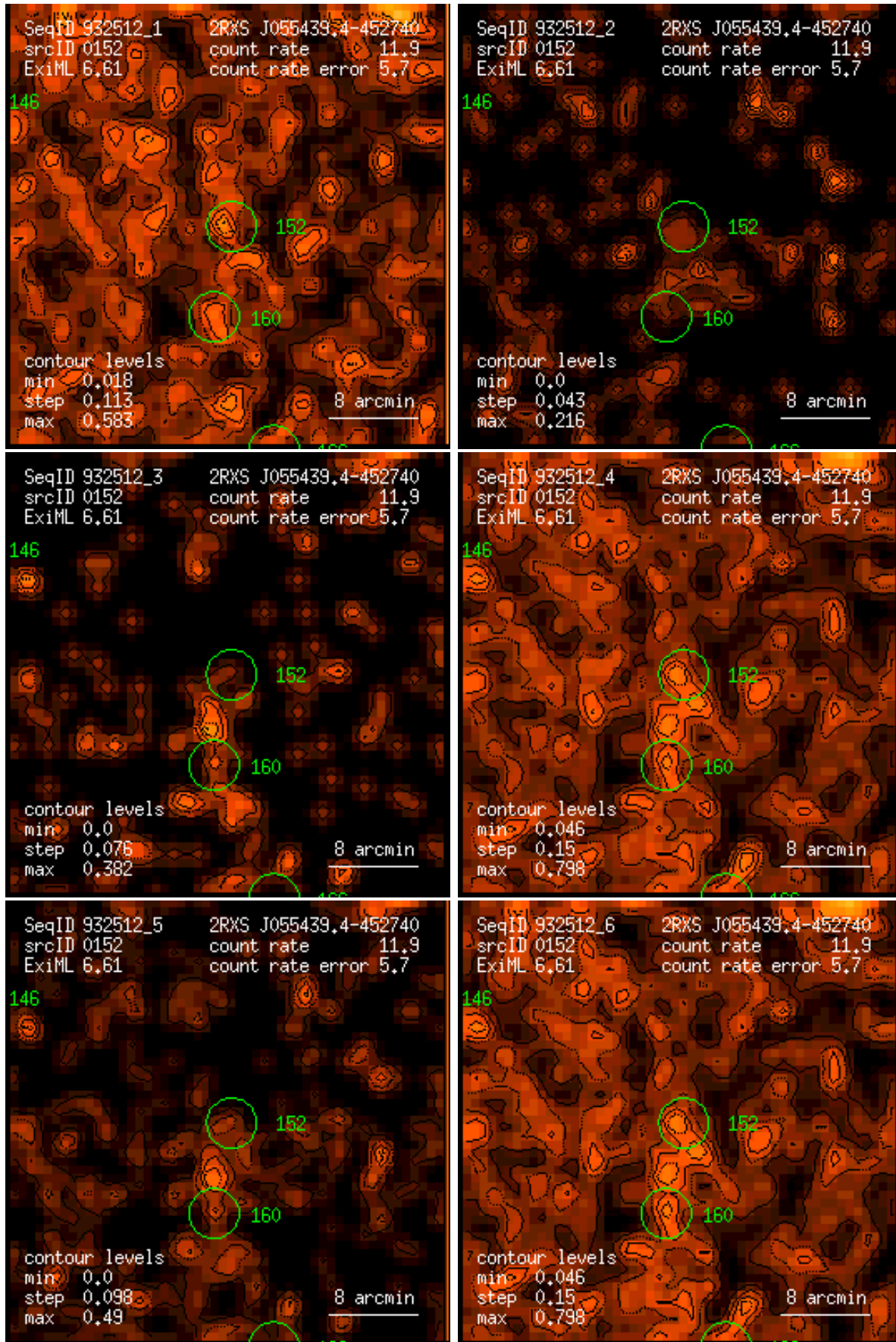
Figure 152: RASS 932512: detection 0152: band rate images, Gaussian filter: (1) PSPC channels 11 – 41, (2) 52 – 90, (3) 91 – 201, (4) 11 – 235, (5) 52 – 201, (6) 11 – 201. Broad band rates in counts/ks. Band rate contour levels in counts/ks/arcmin 2 .
