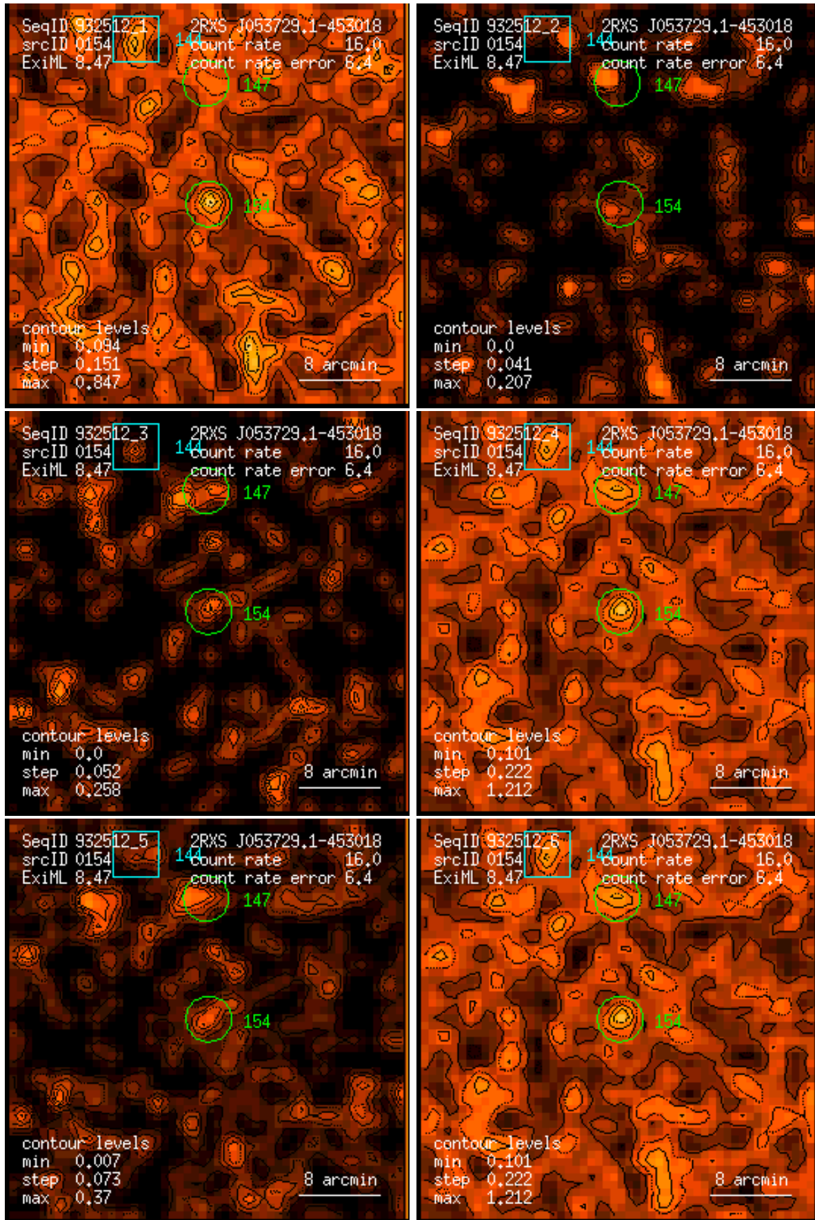
Figure 154: RASS 932512: detection 0154: band rate images, Gaussian filter: (1) PSPC channels 11 – 41, (2) 52 – 90, (3) 91 – 201, (4) 11 – 235, (5) 52 – 201, (6) 11 – 201. Broad band rates in counts/ks. Band rate contour levels in counts/ks/arcmin 2 .
