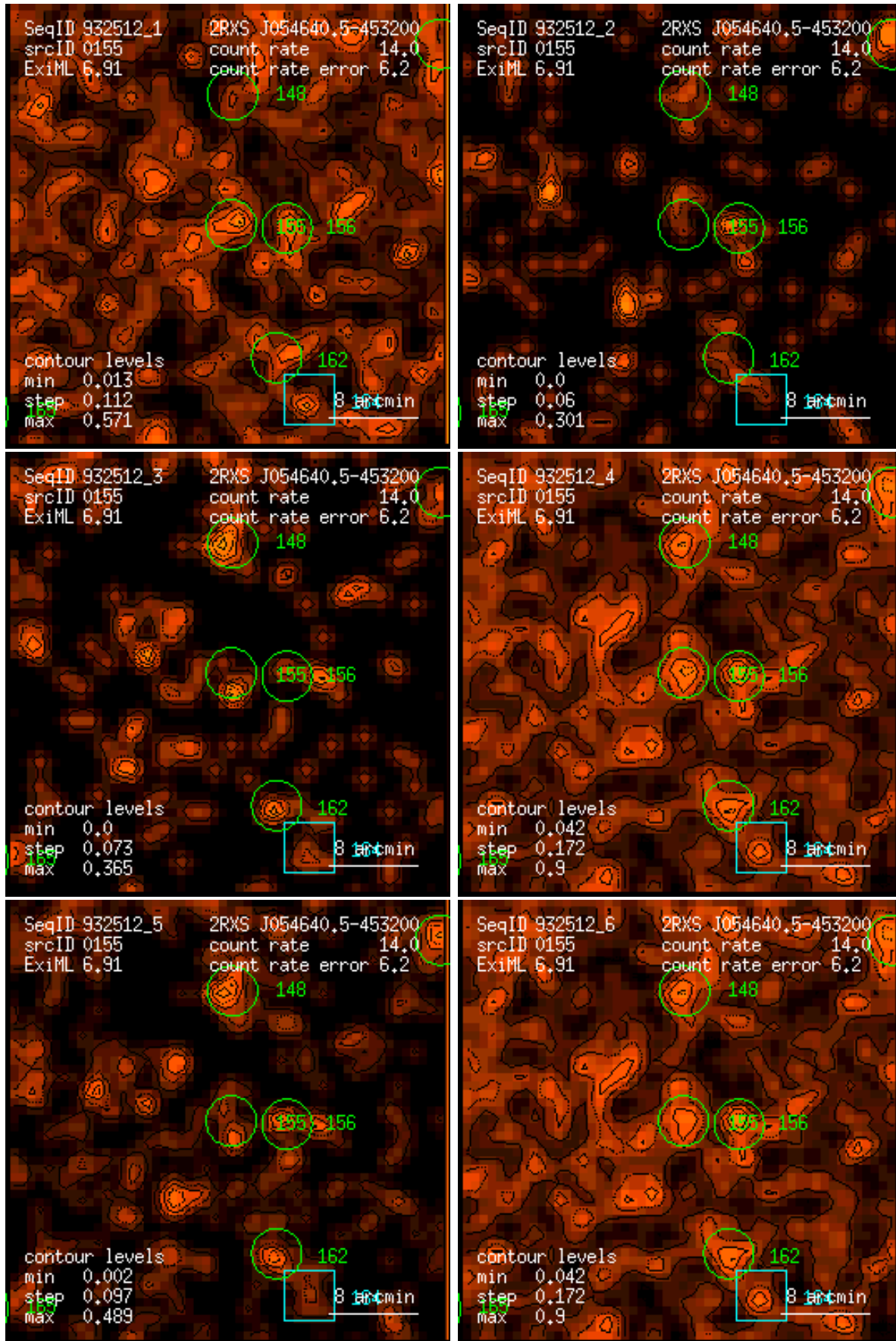
Figure 155: RASS 932512: detection 0155: band rate images, Gaussian filter: (1) PSPC channels 11 – 41, (2) 52 – 90, (3) 91 – 201, (4) 11 – 235, (5) 52 – 201, (6) 11 – 201. Broad band rates in counts/ks. Band rate contour levels in counts/ks/arcmin 2 .
