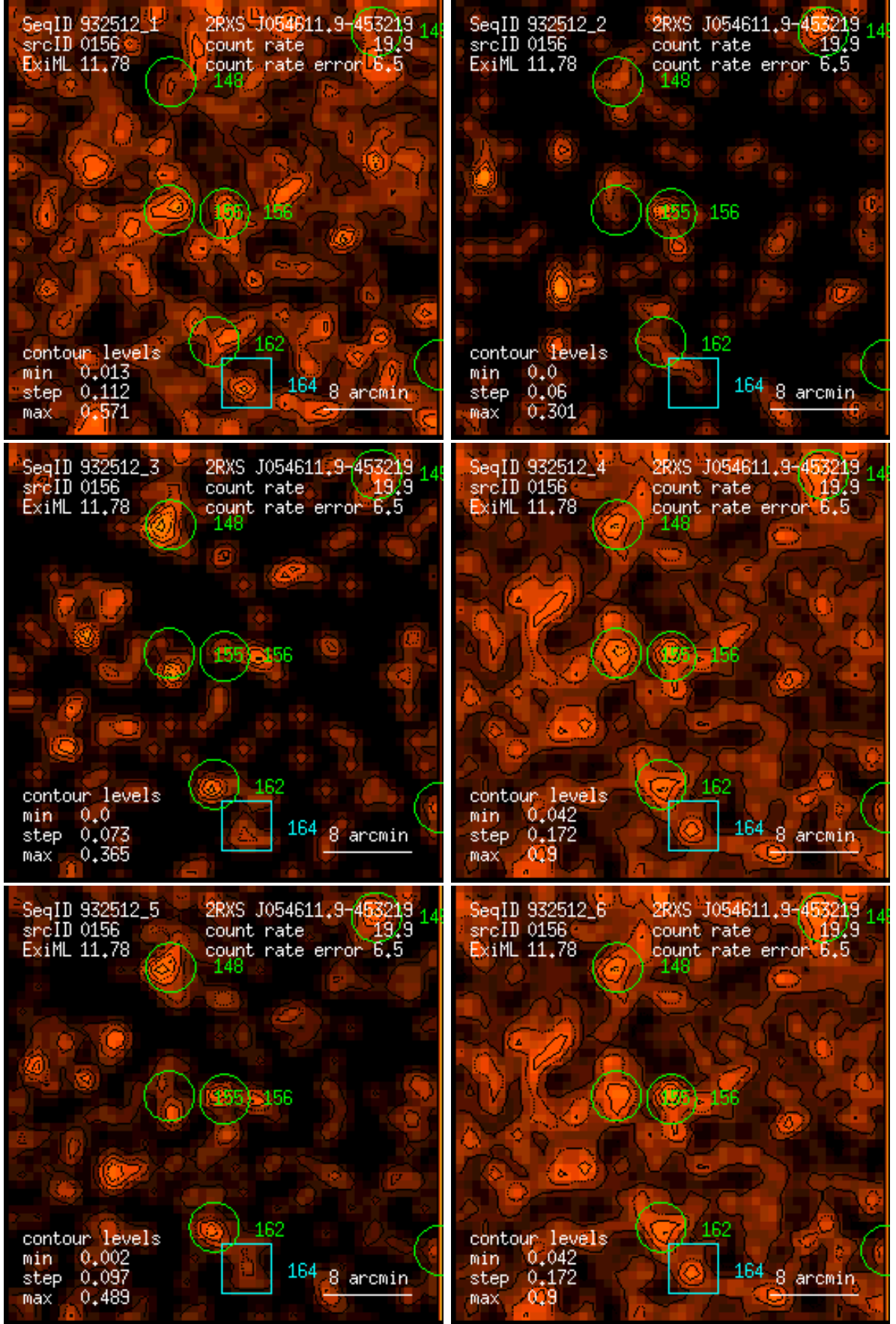
Figure 156: RASS 932512: detection 0156: band rate images, Gaussian filter: (1) PSPC channels 11 – 41, (2) 52 – 90, (3) 91 – 201, (4) 11 – 235, (5) 52 – 201, (6) 11 – 201. Broad band rates in counts/ks. Band rate contour levels in counts/ks/arcmin 2 .
