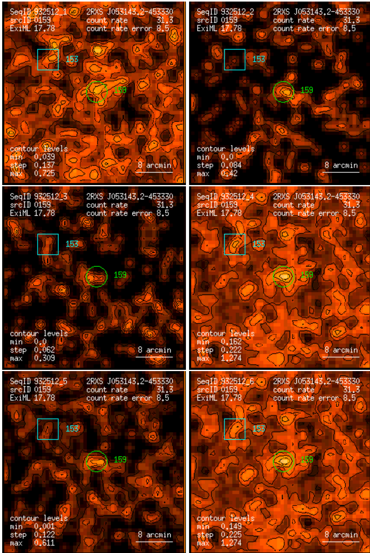
Figure 159: RASS 932512: detection 0159: band rate images, Gaussian filter: (1) PSPC channels 11 – 41, (2) 52 – 90, (3) 91 – 201, (4) 11 – 235, (5) 52 – 201, (6) 11 – 201. Broad band rates in counts/ks. Band rate contour levels in counts/ks/arcmin 2 .
