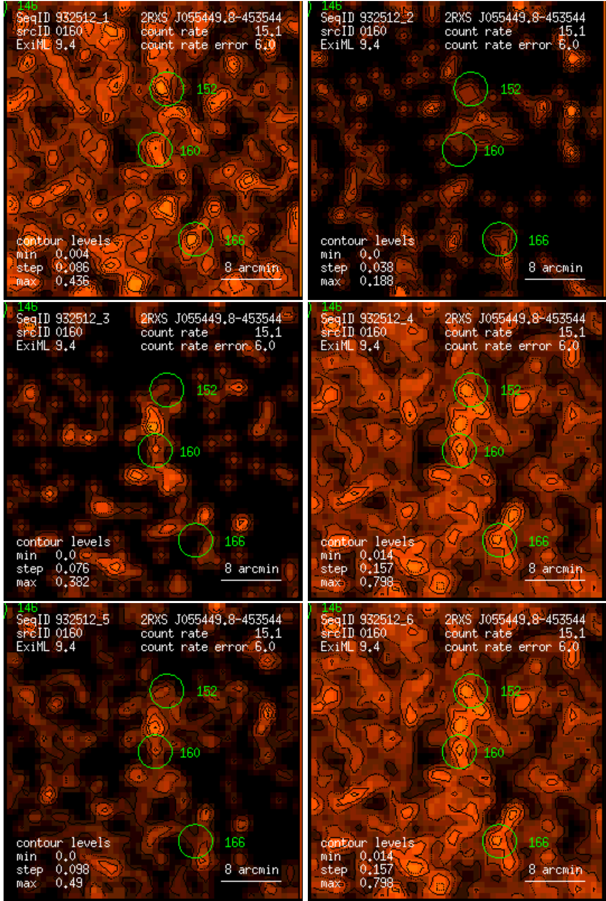
Figure 160: RASS 932512: detection 0160: band rate images, Gaussian filter: (1) PSPC channels 11 – 41, (2) 52 – 90, (3) 91 – 201, (4) 11 – 235, (5) 52 – 201, (6) 11 – 201. Broad band rates in counts/ks. Band rate contour levels in counts/ks/arcmin 2 .
