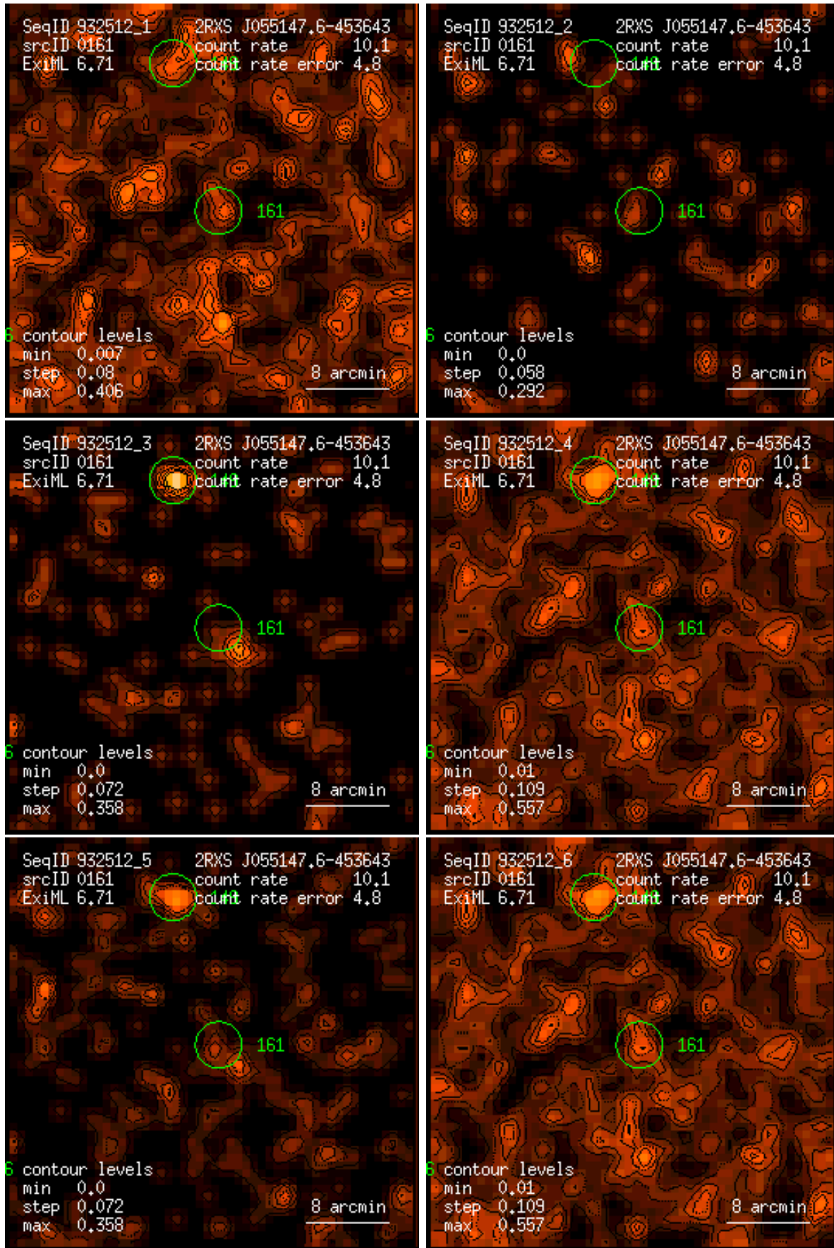
Figure 161: RASS 932512: detection 0161: band rate images, Gaussian filter: (1) PSPC channels 11 – 41, (2) 52 – 90, (3) 91 – 201, (4) 11 – 235, (5) 52 – 201, (6) 11 – 201. Broad band rates in counts/ks. Band rate contour levels in counts/ks/arcmin 2 .
