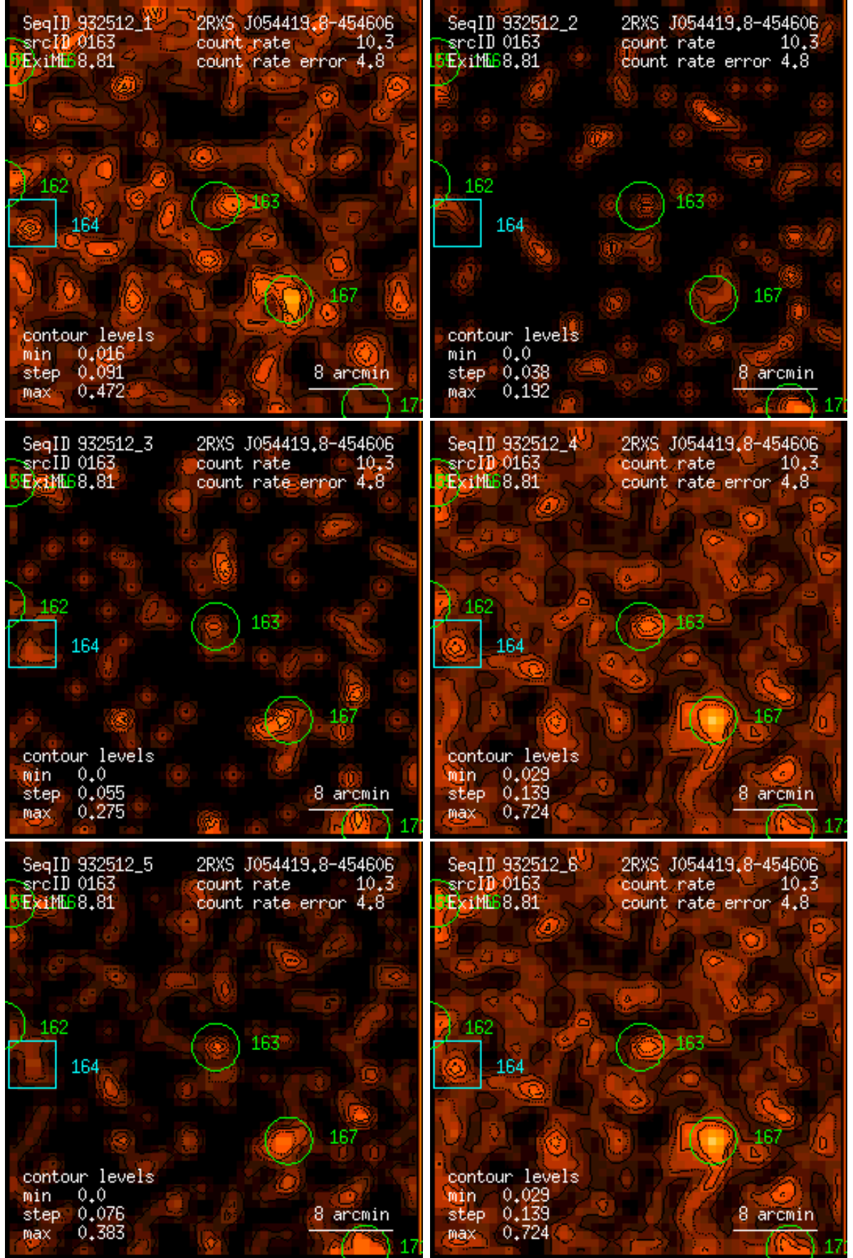
Figure 163: RASS 932512: detection 0163: band rate images, Gaussian filter: (1) PSPC channels 11 – 41, (2) 52 – 90, (3) 91 – 201, (4) 11 – 235, (5) 52 – 201, (6) 11 – 201. Broad band rates in counts/ks. Band rate contour levels in counts/ks/arcmin 2 .
