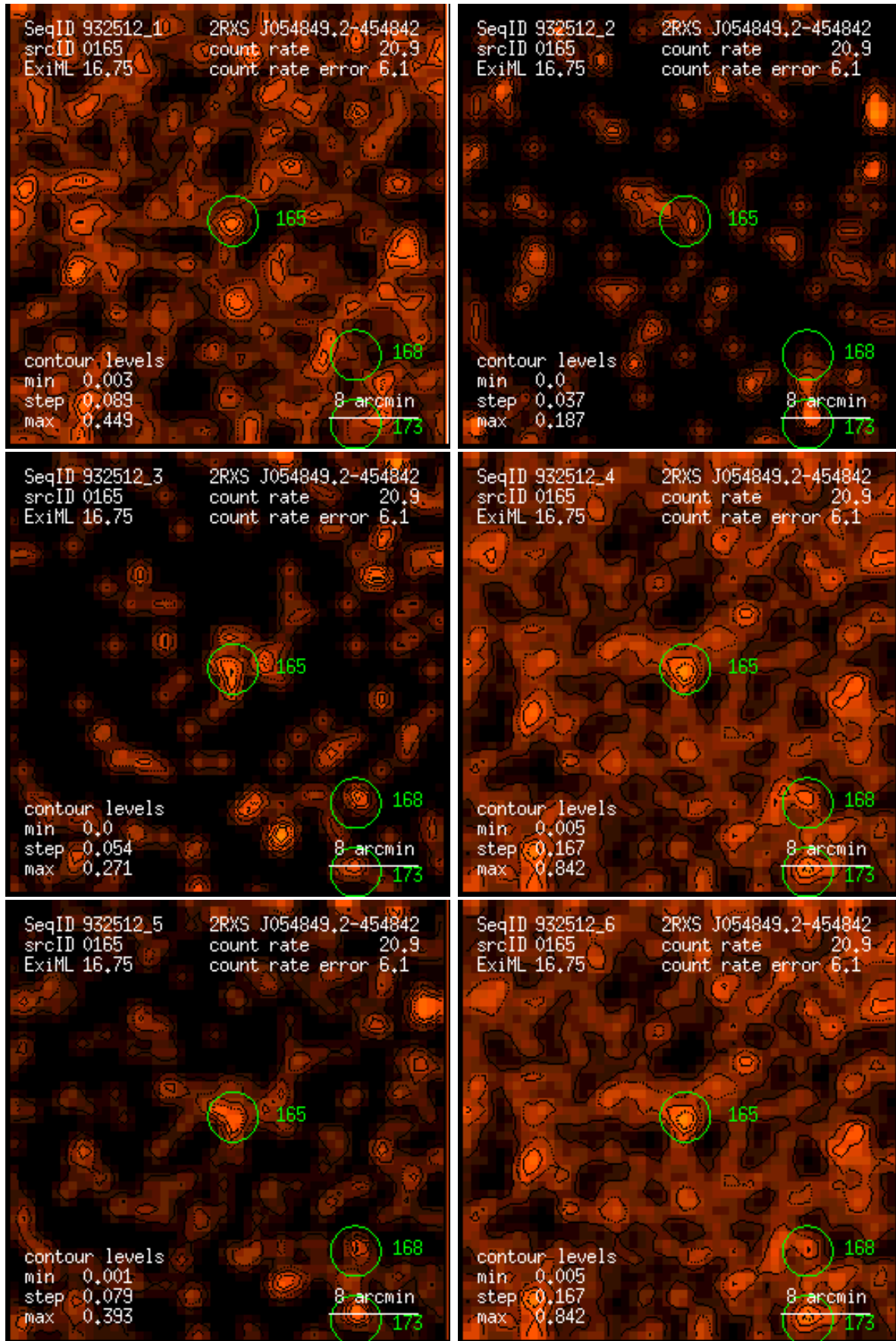
Figure 165: RASS 932512: detection 0165: band rate images, Gaussian filter: (1) PSPC channels 11 – 41, (2) 52 – 90, (3) 91 – 201, (4) 11 – 235, (5) 52 – 201, (6) 11 – 201. Broad band rates in counts/ks. Band rate contour levels in counts/ks/arcmin 2 .
