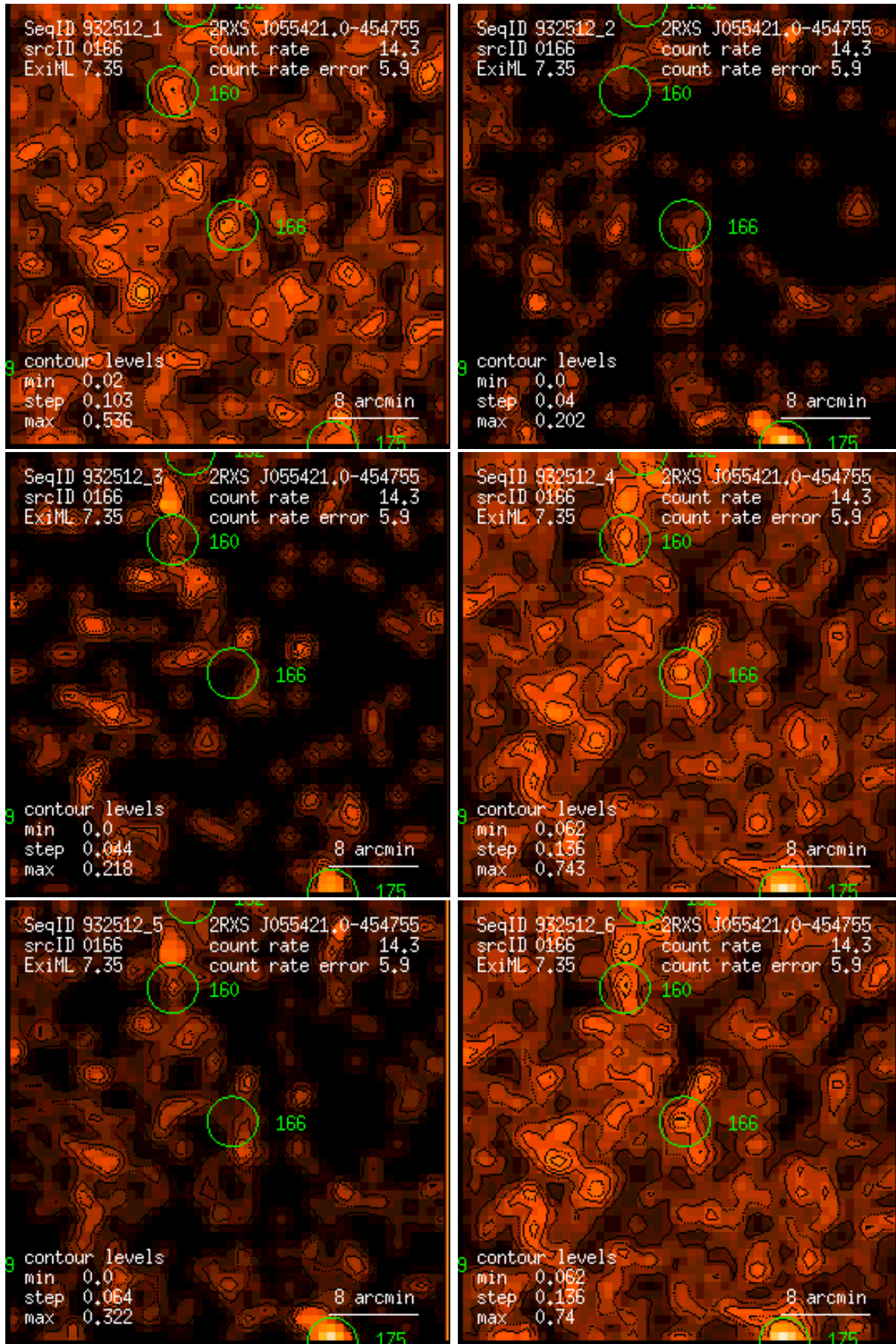
Figure 166: RASS 932512: detection 0166: band rate images, Gaussian filter: (1) PSPC channels 11 – 41, (2) 52 – 90, (3) 91 – 201, (4) 11 – 235, (5) 52 – 201, (6) 11 – 201. Broad band rates in counts/ks. Band rate contour levels in counts/ks/arcmin 2 .
