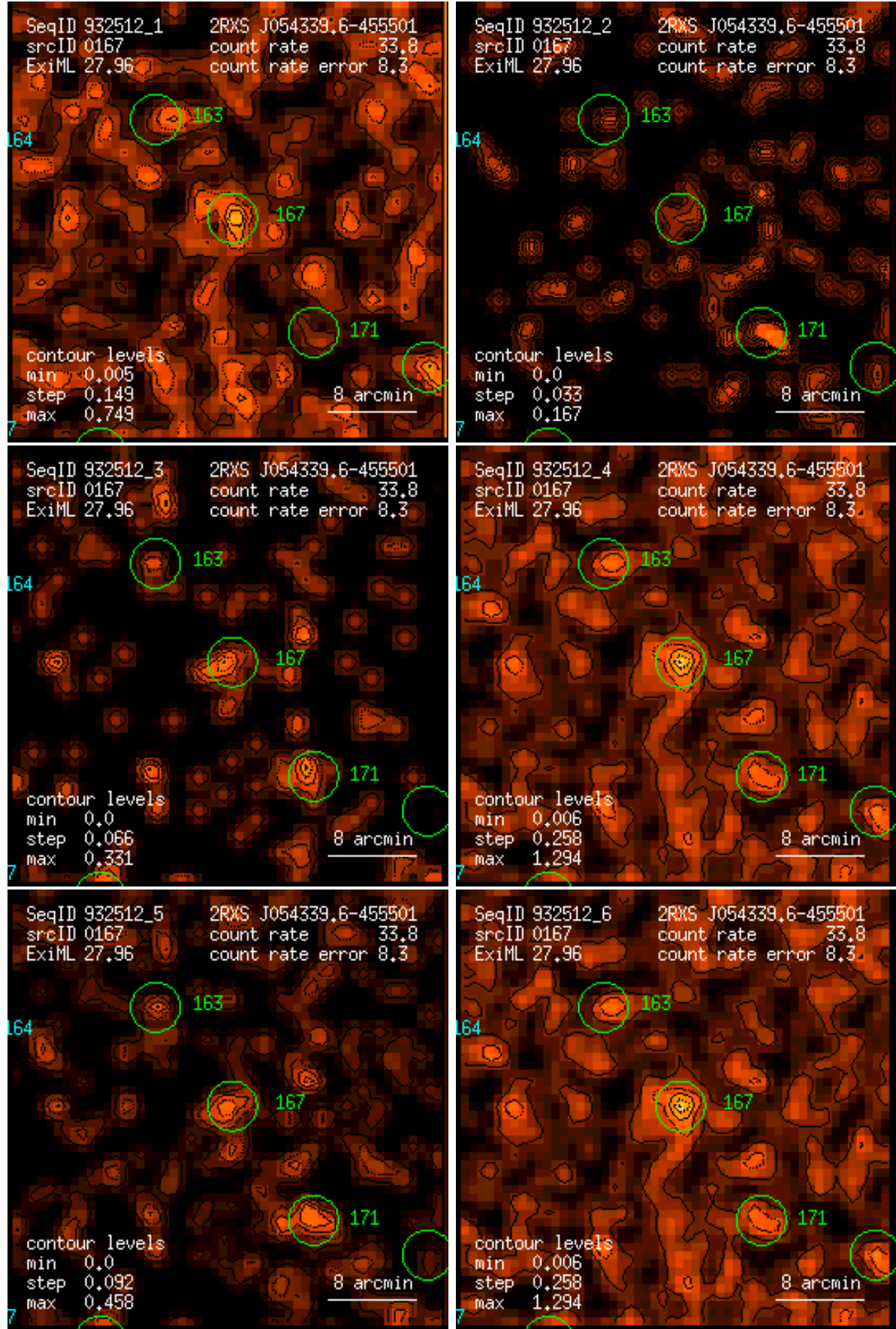
Figure 167: RASS 932512: detection 0167: band rate images, Gaussian filter: (1) PSPC channels 11 – 41, (2) 52 – 90, (3) 91 – 201, (4) 11 – 235, (5) 52 – 201, (6) 11 – 201. Broad band rates in counts/ks. Band rate contour levels in counts/ks/arcmin 2 .
