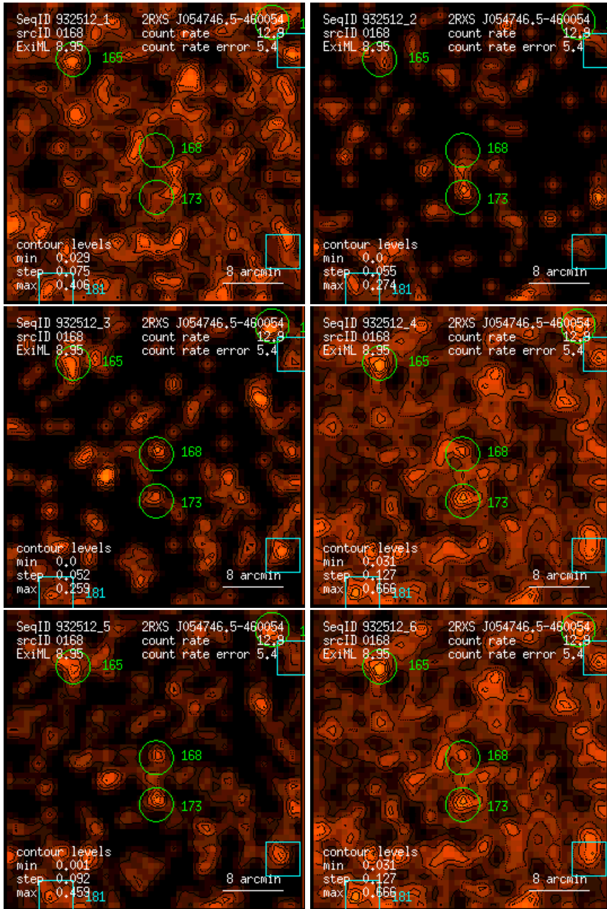
Figure 168: RASS 932512: detection 0168: band rate images, Gaussian filter: (1) PSPC channels 11 – 41, (2) 52 – 90, (3) 91 – 201, (4) 11 – 235, (5) 52 – 201, (6) 11 – 201. Broad band rates in counts/ks. Band rate contour levels in counts/ks/arcmin 2 .
