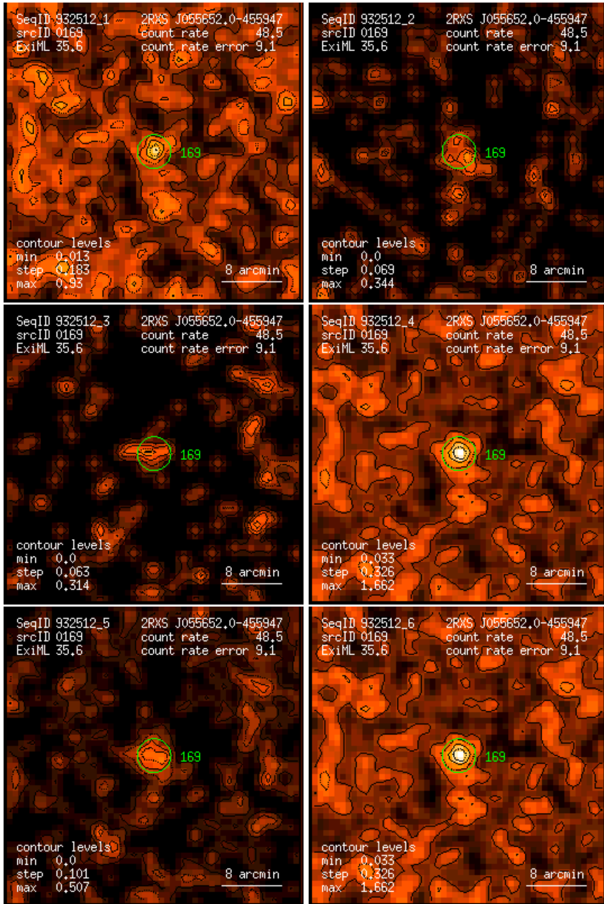
Figure 169: RASS 932512: detection 0169: band rate images, Gaussian filter: (1) PSPC channels 11 – 41, (2) 52 – 90, (3) 91 – 201, (4) 11 – 235, (5) 52 – 201, (6) 11 – 201. Broad band rates in counts/ks. Band rate contour levels in counts/ks/arcmin 2 .
