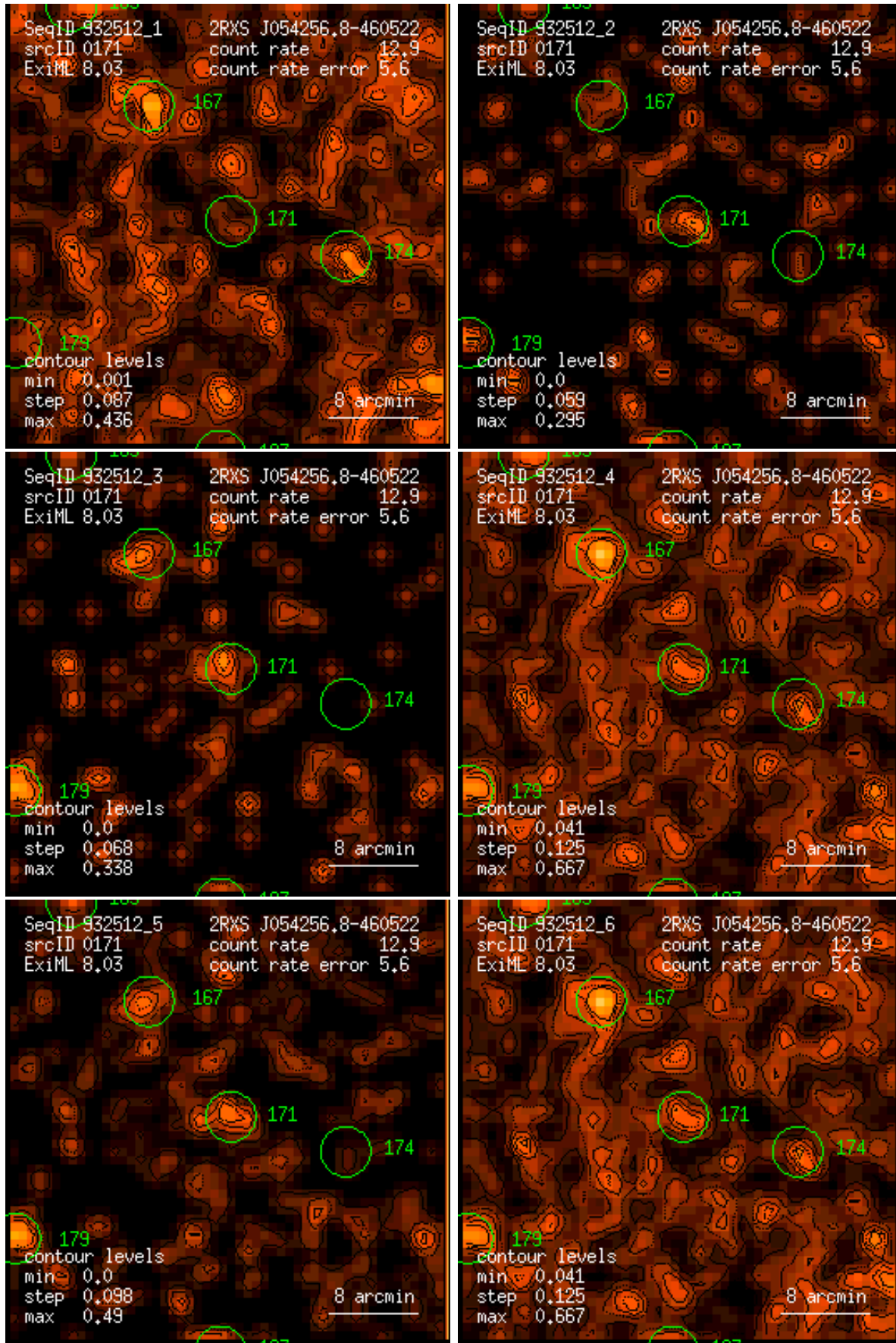
Figure 171: RASS 932512: detection 0171: band rate images, Gaussian filter: (1) PSPC channels 11 – 41, (2) 52 – 90, (3) 91 – 201, (4) 11 – 235, (5) 52 – 201, (6) 11 – 201. Broad band rates in counts/ks. Band rate contour levels in counts/ks/arcmin 2 .
