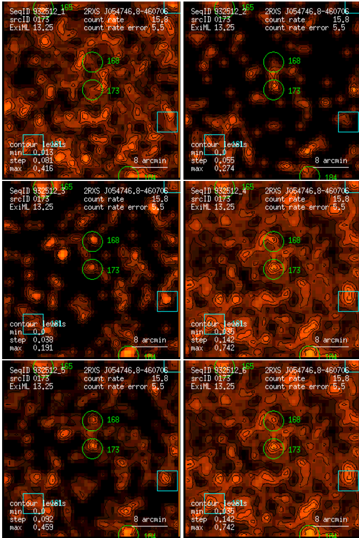
Figure 173: RASS 932512: detection 0173: band rate images, Gaussian filter: (1) PSPC channels 11 – 41, (2) 52 – 90, (3) 91 – 201, (4) 11 – 235, (5) 52 – 201, (6) 11 – 201. Broad band rates in counts/ks. Band rate contour levels in counts/ks/arcmin 2 .
