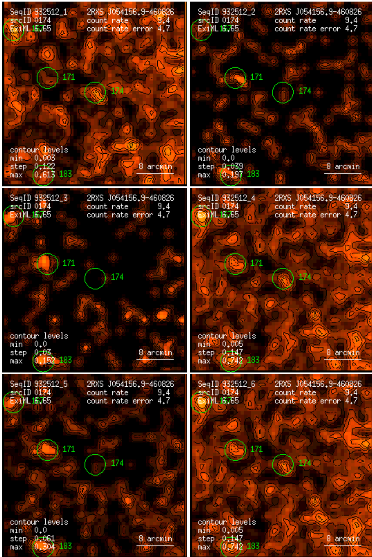
Figure 174: RASS 932512: detection 0174: band rate images, Gaussian filter: (1) PSPC channels 11 – 41, (2) 52 – 90, (3) 91 – 201, (4) 11 – 235, (5) 52 – 201, (6) 11 – 201. Broad band rates in counts/ks. Band rate contour levels in counts/ks/arcmin 2 .
