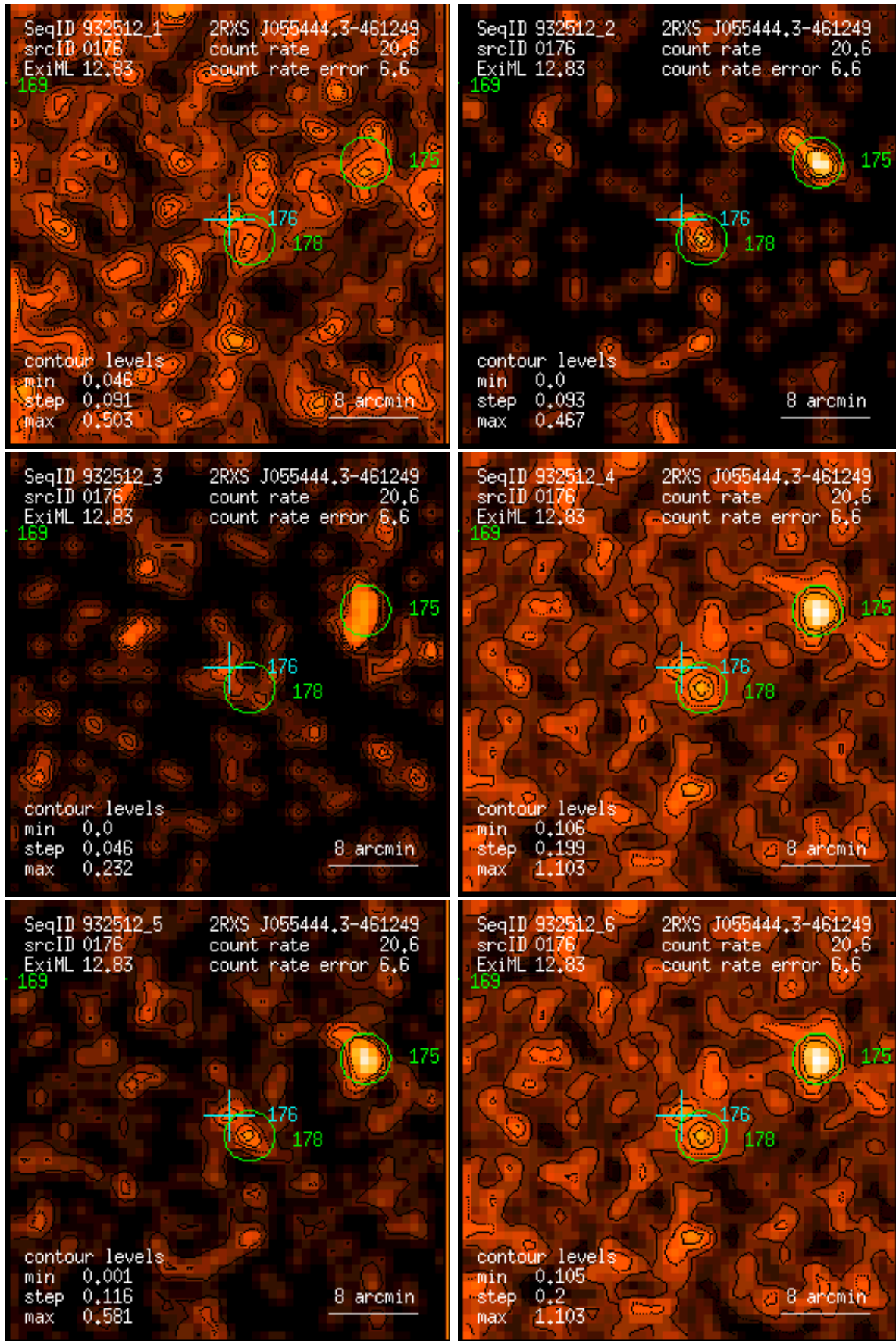
Figure 176: RASS 932512: detection 0176: band rate images, Gaussian filter: (1) PSPC channels 11 – 41, (2) 52 – 90, (3) 91 – 201, (4) 11 – 235, (5) 52 – 201, (6) 11 – 201. Broad band rates in counts/ks. Band rate contour levels in counts/ks/arcmin 2 .
