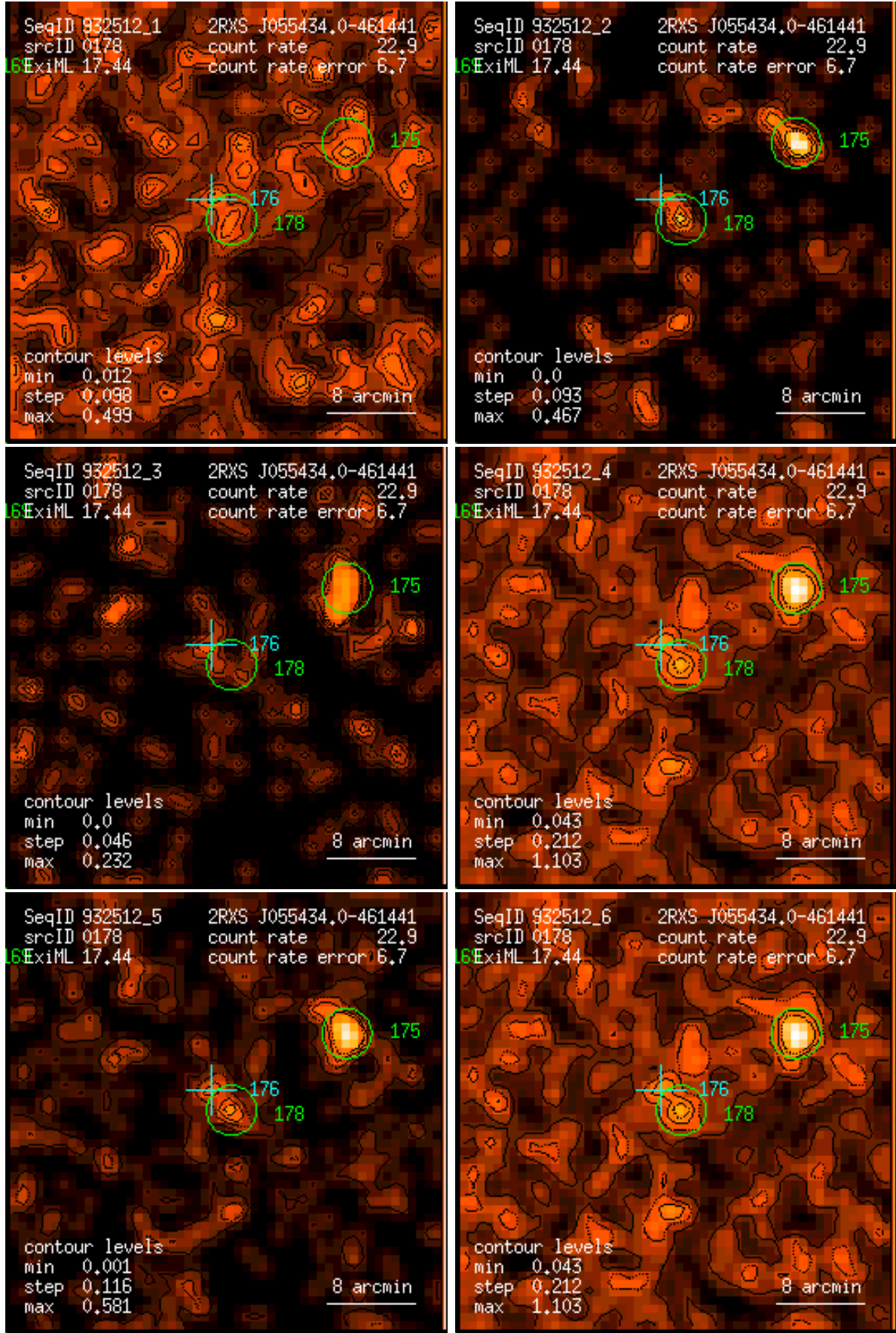
Figure 178: RASS 932512: detection 0178: band rate images, Gaussian filter: (1) PSPC channels 11 – 41, (2) 52 – 90, (3) 91 – 201, (4) 11 – 235, (5) 52 – 201, (6) 11 – 201. Broad band rates in counts/ks. Band rate contour levels in counts/ks/arcmin 2 .
