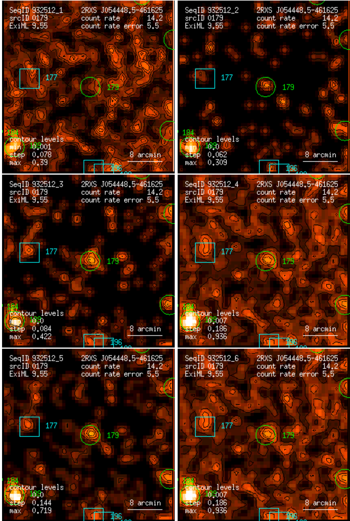
Figure 179: RASS 932512: detection 0179: band rate images, Gaussian filter: (1) PSPC channels 11 – 41, (2) 52 – 90, (3) 91 – 201, (4) 11 – 235, (5) 52 – 201, (6) 11 – 201. Broad band rates in counts/ks. Band rate contour levels in counts/ks/arcmin 2 .
