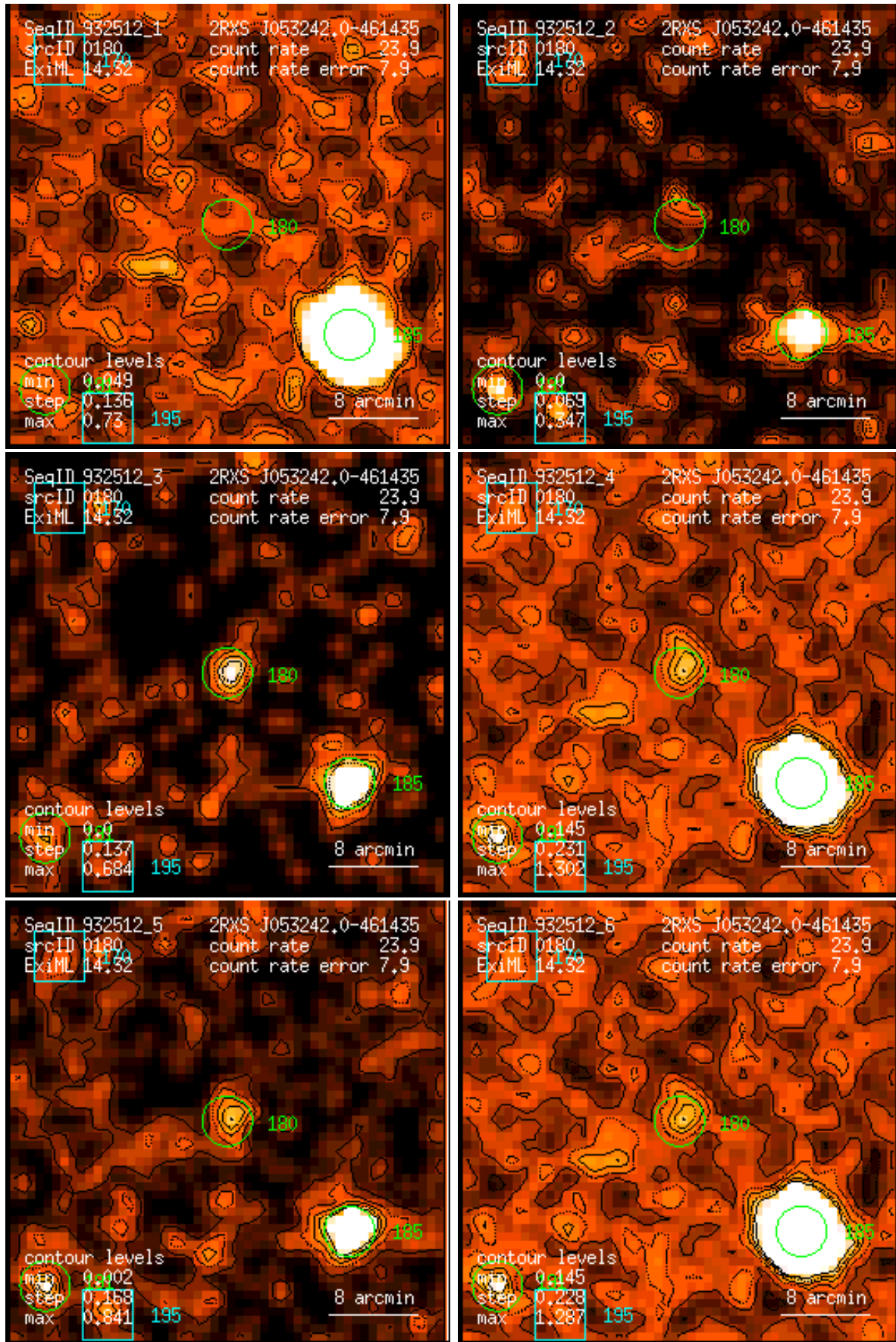
Figure 180: RASS 932512: detection 0180: band rate images, Gaussian filter: (1) PSPC channels 11 – 41, (2) 52 – 90, (3) 91 – 201, (4) 11 – 235, (5) 52 – 201, (6) 11 – 201. Broad band rates in counts/ks. Band rate contour levels in counts/ks/arcmin 2 .
