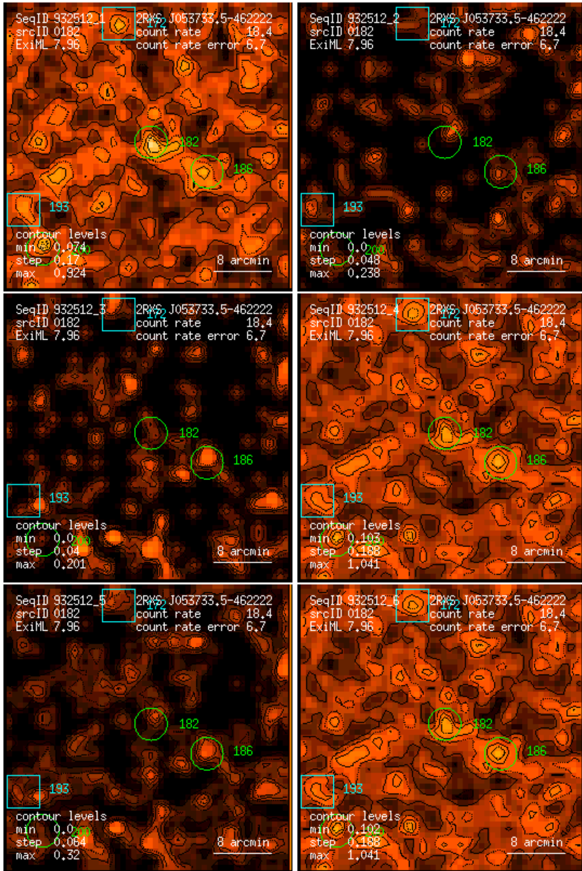
Figure 182: RASS 932512: detection 0182: band rate images, Gaussian filter: (1) PSPC channels 11 – 41, (2) 52 – 90, (3) 91 – 201, (4) 11 – 235, (5) 52 – 201, (6) 11 – 201. Broad band rates in counts/ks. Band rate contour levels in counts/ks/arcmin 2 .
