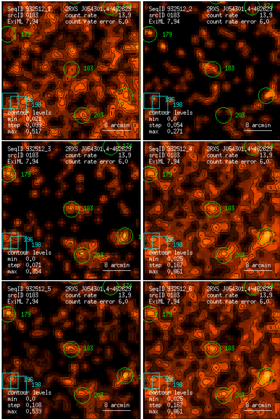
Figure 183: RASS 932512: detection 0183: band rate images, Gaussian filter: (1) PSPC channels 11 – 41, (2) 52 – 90, (3) 91 – 201, (4) 11 – 235, (5) 52 – 201, (6) 11 – 201. Broad band rates in counts/ks. Band rate contour levels in counts/ks/arcmin 2 .
