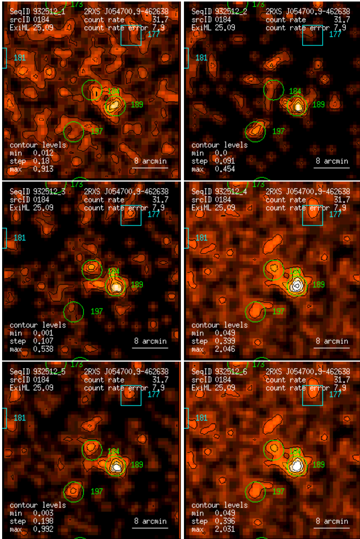
Figure 184: RASS 932512: detection 0184: band rate images, Gaussian filter: (1) PSPC channels 11 – 41, (2) 52 – 90, (3) 91 – 201, (4) 11 – 235, (5) 52 – 201, (6) 11 – 201. Broad band rates in counts/ks. Band rate contour levels in counts/ks/arcmin 2 .
