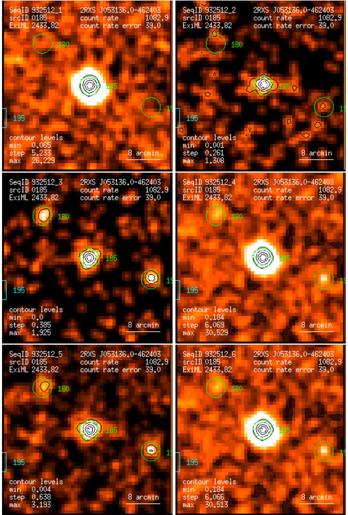
Figure 185: RASS 932512: detection 0185: band rate images, Gaussian filter: (1) PSPC channels 11 – 41, (2) 52 – 90, (3) 91 – 201, (4) 11 – 235, (5) 52 – 201, (6) 11 – 201. Broad band rates in counts/ks. Band rate contour levels in counts/ks/arcmin 2 .
