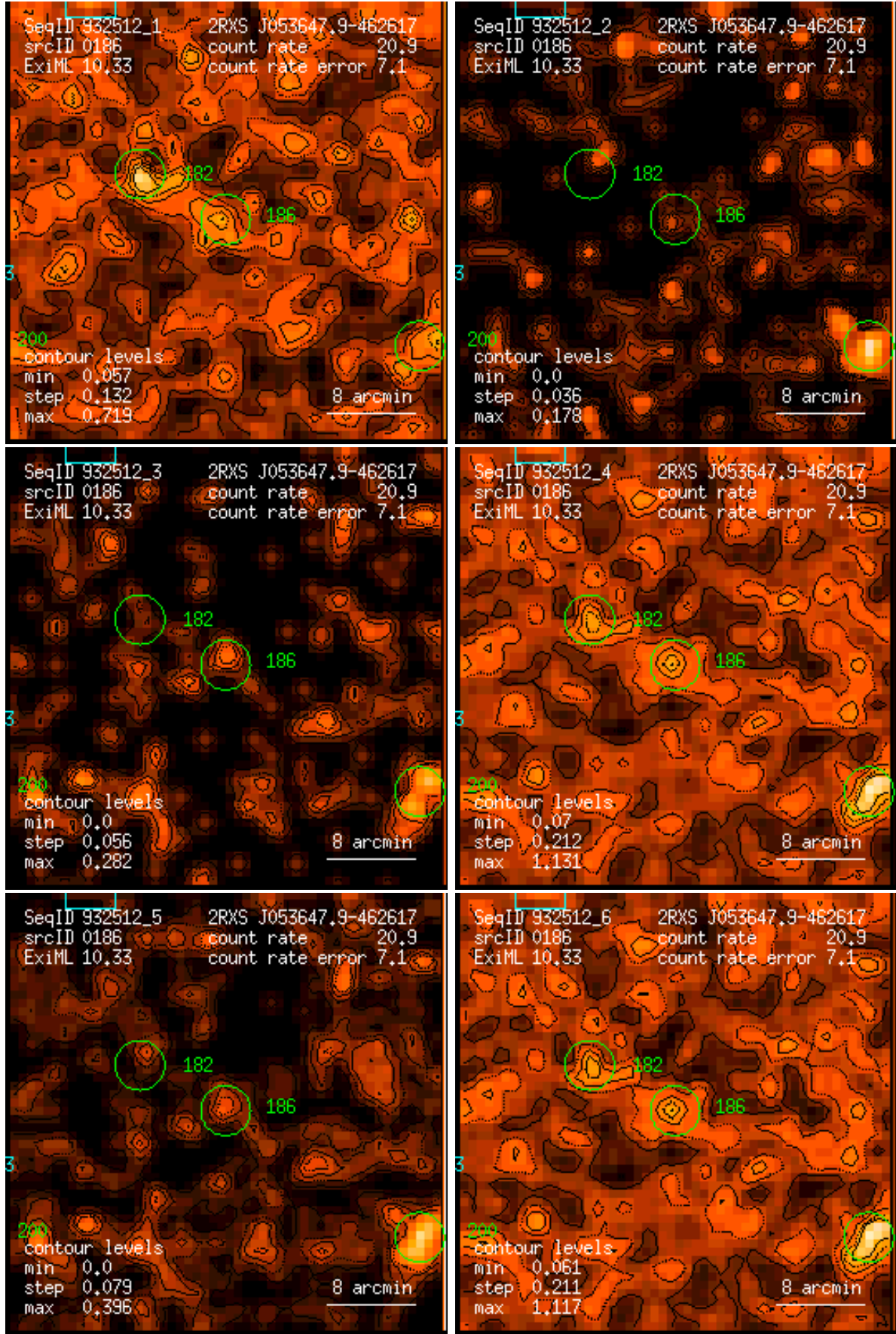
Figure 186: RASS 932512: detection 0186: band rate images, Gaussian filter: (1) PSPC channels 11 – 41, (2) 52 – 90, (3) 91 – 201, (4) 11 – 235, (5) 52 – 201, (6) 11 – 201. Broad band rates in counts/ks. Band rate contour levels in counts/ks/arcmin 2 .
