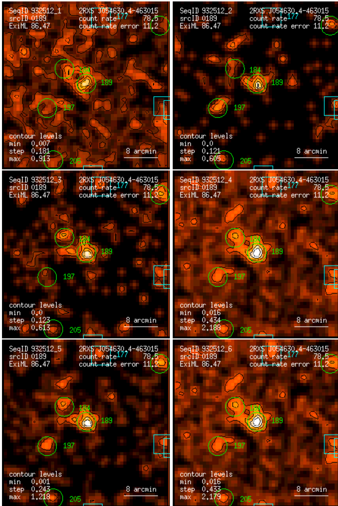
Figure 189: RASS 932512: detection 0189: band rate images, Gaussian filter: (1) PSPC channels 11 – 41, (2) 52 – 90, (3) 91 – 201, (4) 11 – 235, (5) 52 – 201, (6) 11 – 201. Broad band rates in counts/ks. Band rate contour levels in counts/ks/arcmin 2 .
