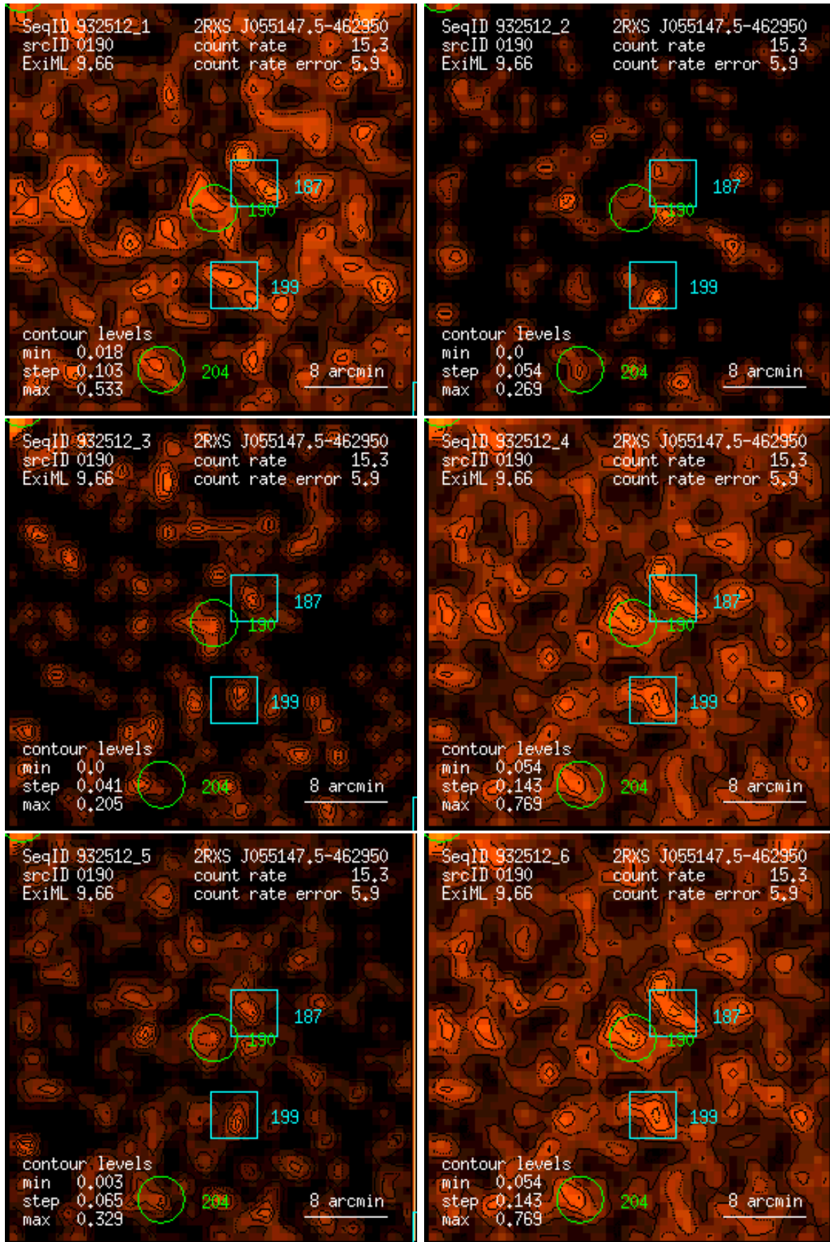
Figure 190: RASS 932512: detection 0190: band rate images, Gaussian filter: (1) PSPC channels 11 – 41, (2) 52 – 90, (3) 91 – 201, (4) 11 – 235, (5) 52 – 201, (6) 11 – 201. Broad band rates in counts/ks. Band rate contour levels in counts/ks/arcmin 2 .
