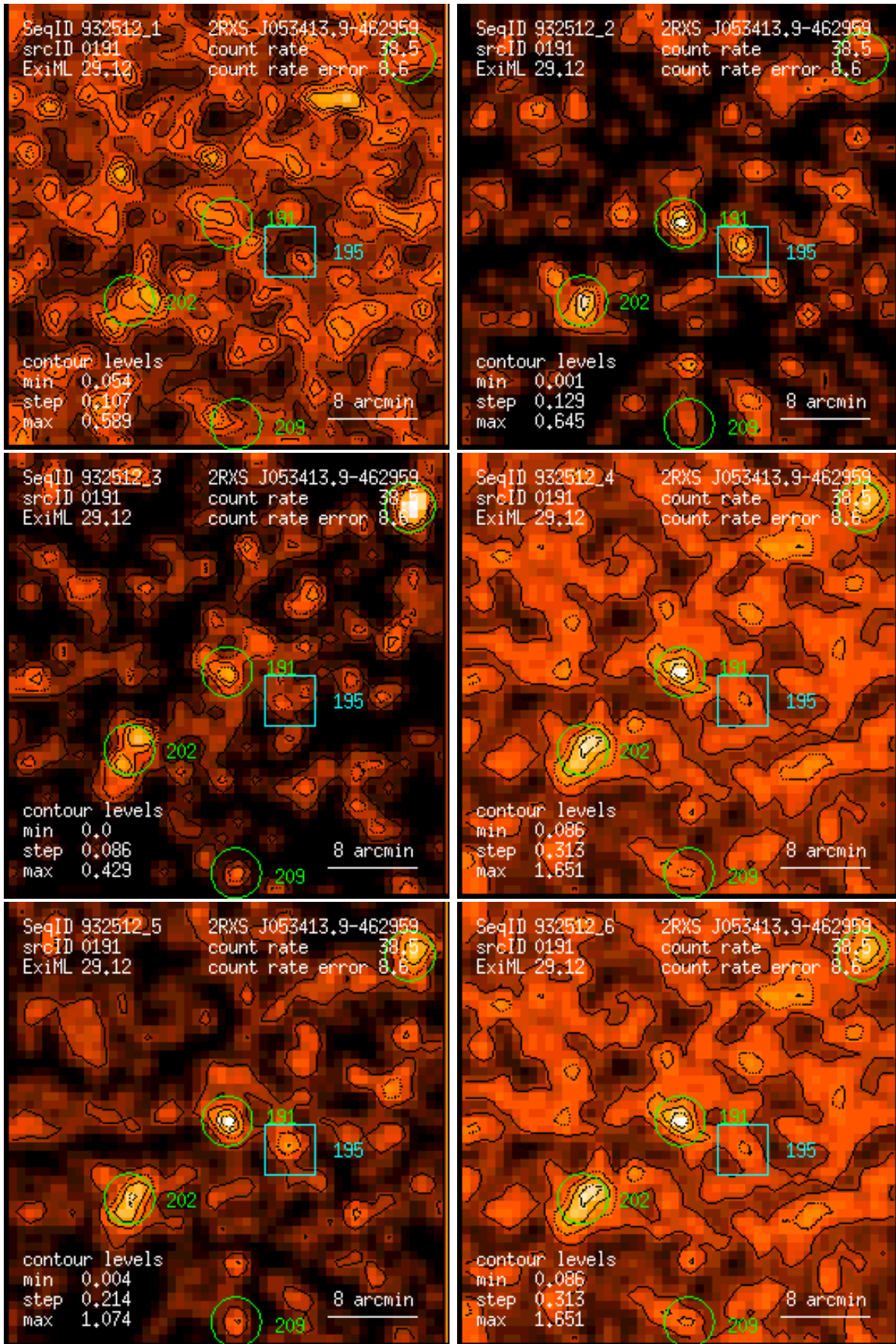
Figure 191: RASS 932512: detection 0191: band rate images, Gaussian filter: (1) PSPC channels 11 – 41, (2) 52 – 90, (3) 91 – 201, (4) 11 – 235, (5) 52 – 201, (6) 11 – 201. Broad band rates in counts/ks. Band rate contour levels in counts/ks/arcmin 2 .
