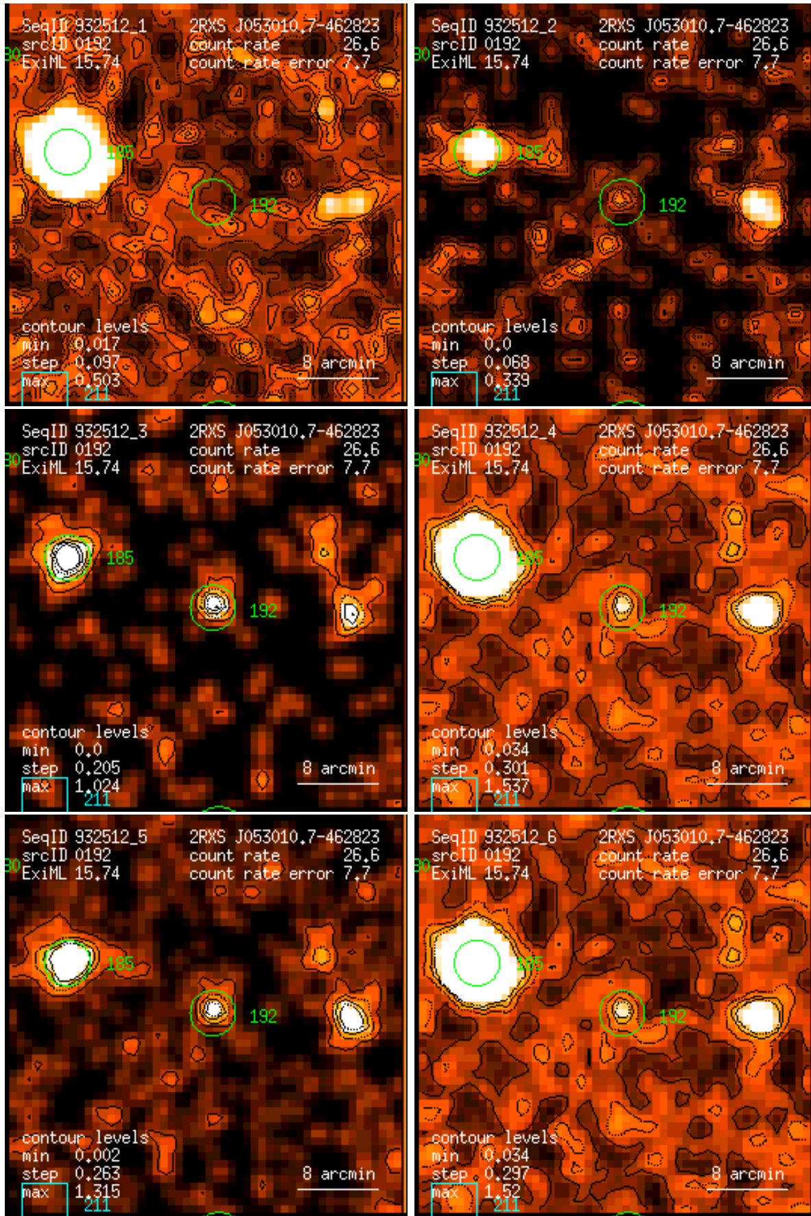
Figure 192: RASS 932512: detection 0192: band rate images, Gaussian filter: (1) PSPC channels 11 – 41, (2) 52 – 90, (3) 91 – 201, (4) 11 – 235, (5) 52 – 201, (6) 11 – 201. Broad band rates in counts/ks. Band rate contour levels in counts/ks/arcmin 2 .
