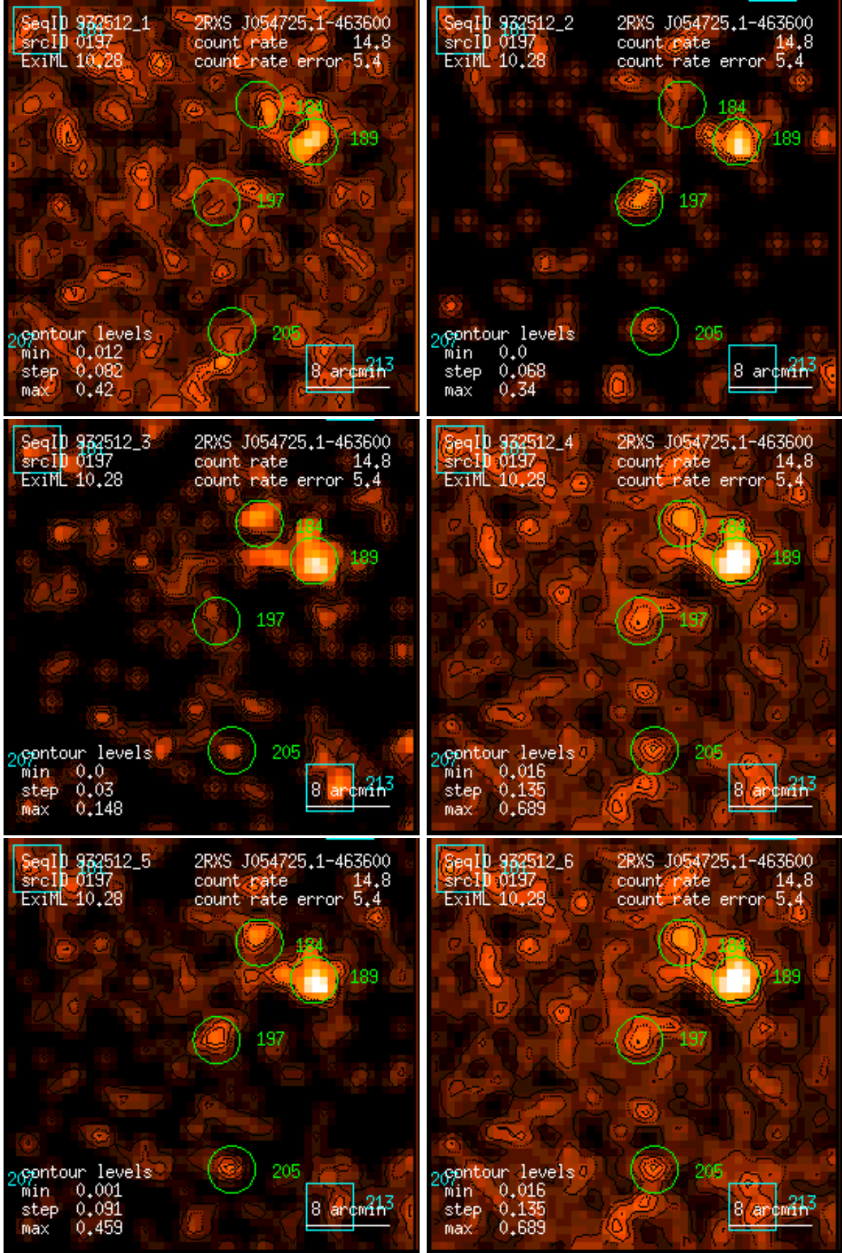
Figure 197: RASS 932512: detection 0197: band rate images, Gaussian filter: (1) PSPC channels 11 – 41, (2) 52 – 90, (3) 91 – 201, (4) 11 – 235, (5) 52 – 201, (6) 11 – 201. Broad band rates in counts/ks. Band rate contour levels in counts/ks/arcmin 2 .
