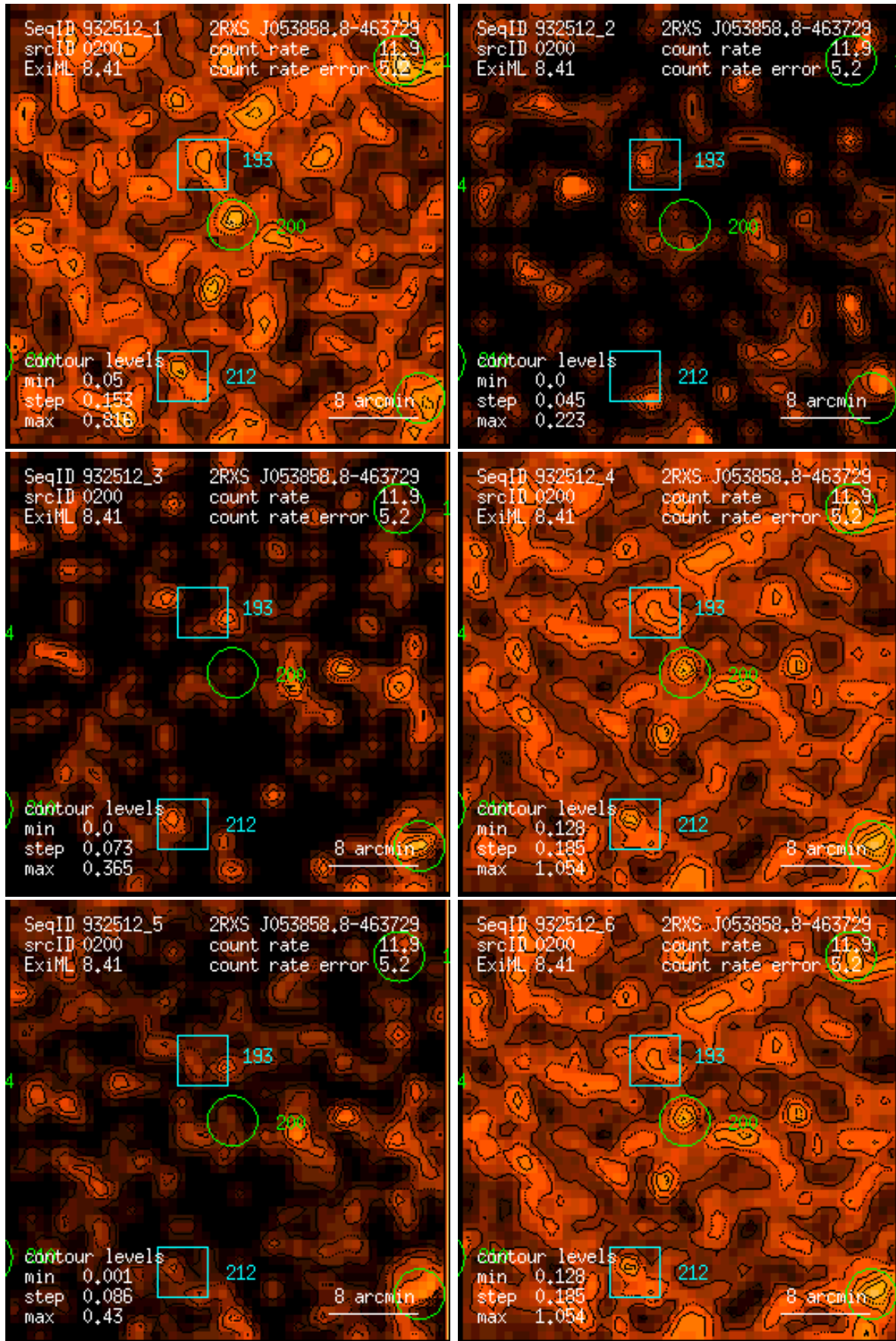
Figure 200: RASS 932512: detection 0200: band rate images, Gaussian filter: (1) PSPC channels 11 – 41, (2) 52 – 90, (3) 91 – 201, (4) 11 – 235, (5) 52 – 201, (6) 11 – 201. Broad band rates in counts/ks. Band rate contour levels in counts/ks/arcmin 2 .
