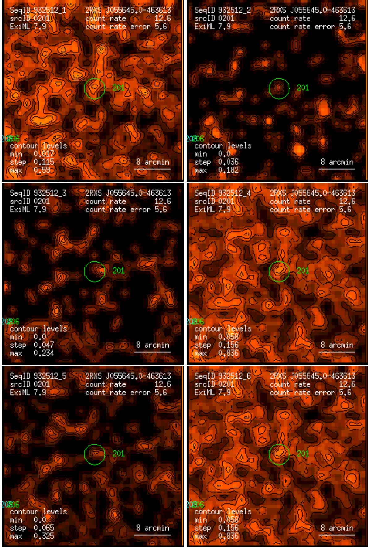
Figure 201: RASS 932512: detection 0201: band rate images, Gaussian filter: (1) PSPC channels 11 – 41, (2) 52 – 90, (3) 91 – 201, (4) 11 – 235, (5) 52 – 201, (6) 11 – 201. Broad band rates in counts/ks. Band rate contour levels in counts/ks/arcmin 2 .
