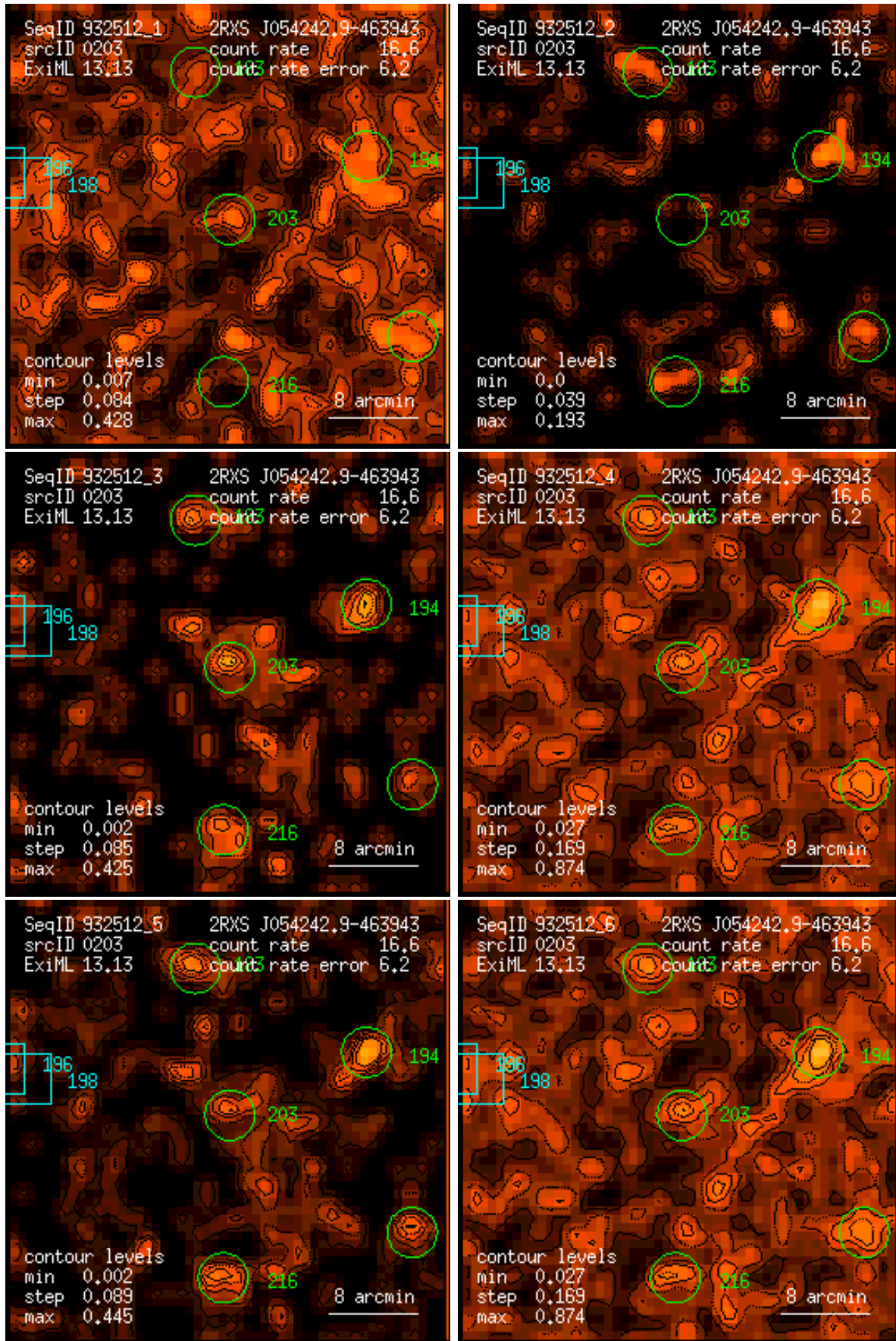
Figure 203: RASS 932512: detection 0203: band rate images, Gaussian filter: (1) PSPC channels 11 – 41, (2) 52 – 90, (3) 91 – 201, (4) 11 – 235, (5) 52 – 201, (6) 11 – 201. Broad band rates in counts/ks. Band rate contour levels in counts/ks/arcmin 2 .
