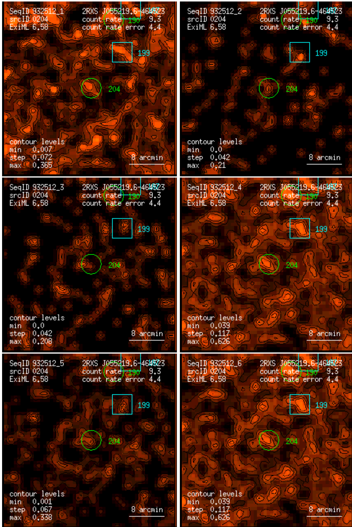
Figure 204: RASS 932512: detection 0204: band rate images, Gaussian filter: (1) PSPC channels 11 – 41, (2) 52 – 90, (3) 91 – 201, (4) 11 – 235, (5) 52 – 201, (6) 11 – 201. Broad band rates in counts/ks. Band rate contour levels in counts/ks/arcmin 2 .
