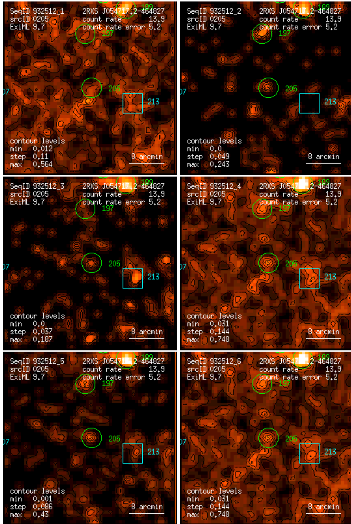
Figure 205: RASS 932512: detection 0205: band rate images, Gaussian filter: (1) PSPC channels 11 – 41, (2) 52 – 90, (3) 91 – 201, (4) 11 – 235, (5) 52 – 201, (6) 11 – 201. Broad band rates in counts/ks. Band rate contour levels in counts/ks/arcmin 2 .
