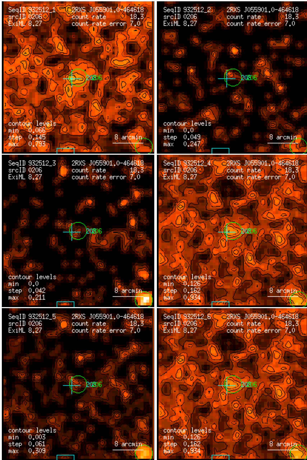
Figure 206: RASS 932512: detection 0206: band rate images, Gaussian filter: (1) PSPC channels 11 – 41, (2) 52 – 90, (3) 91 – 201, (4) 11 – 235, (5) 52 – 201, (6) 11 – 201. Broad band rates in counts/ks. Band rate contour levels in counts/ks/arcmin 2 .
