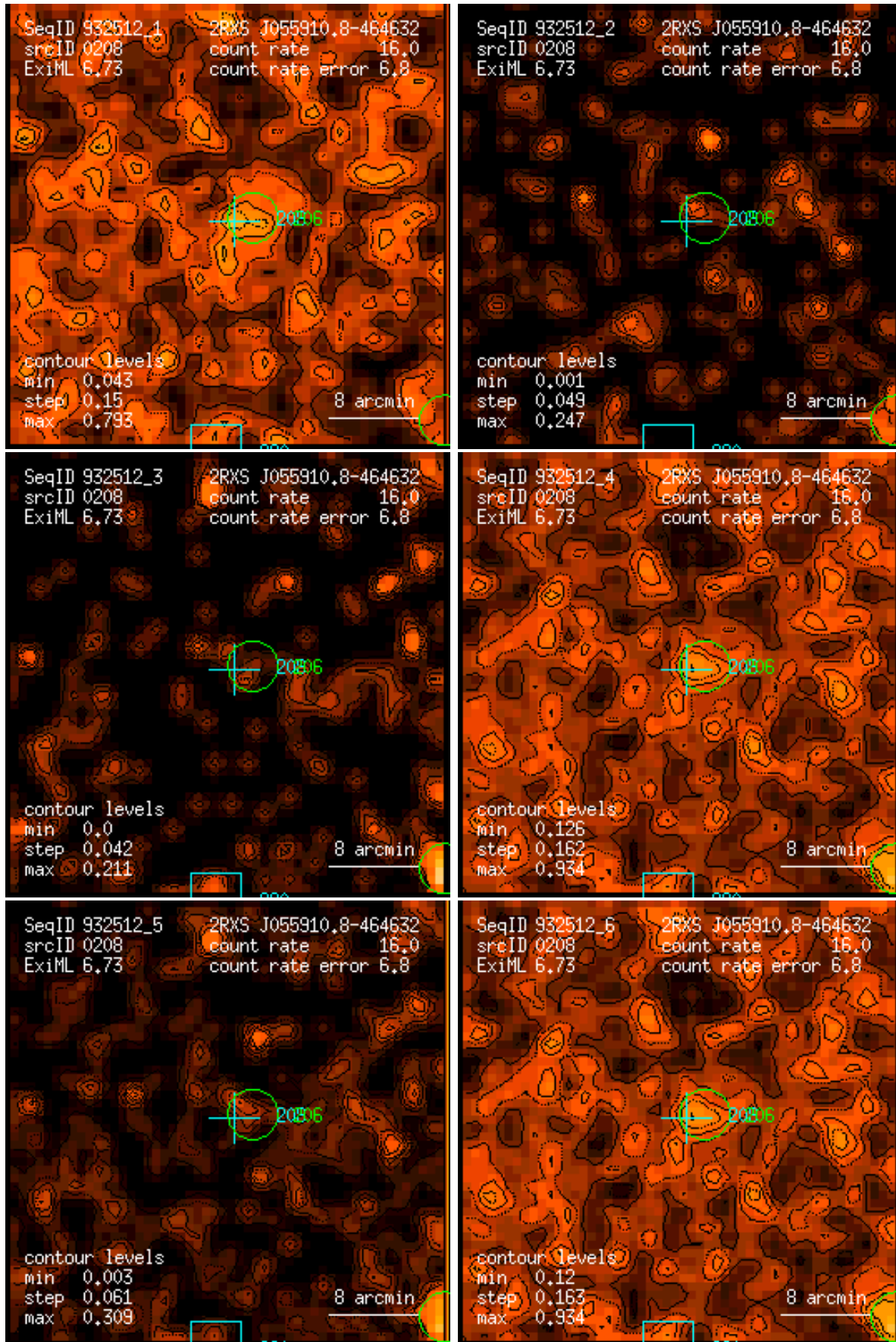
Figure 208: RASS 932512: detection 0208: band rate images, Gaussian filter: (1) PSPC channels 11 – 41, (2) 52 – 90, (3) 91 – 201, (4) 11 – 235, (5) 52 – 201, (6) 11 – 201. Broad band rates in counts/ks. Band rate contour levels in counts/ks/arcmin 2 .
