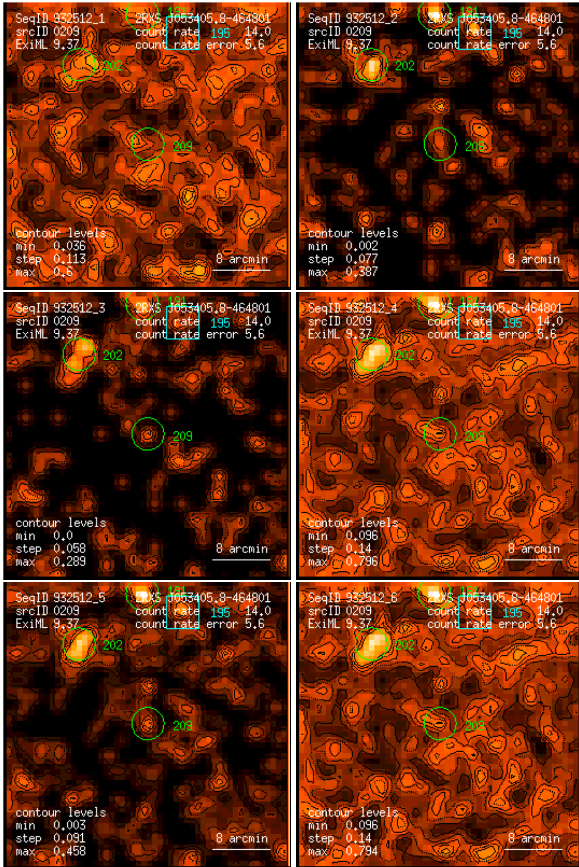
Figure 209: RASS 932512: detection 0209: band rate images, Gaussian filter: (1) PSPC channels 11 – 41, (2) 52 – 90, (3) 91 – 201, (4) 11 – 235, (5) 52 – 201, (6) 11 – 201. Broad band rates in counts/ks. Band rate contour levels in counts/ks/arcmin 2 .
