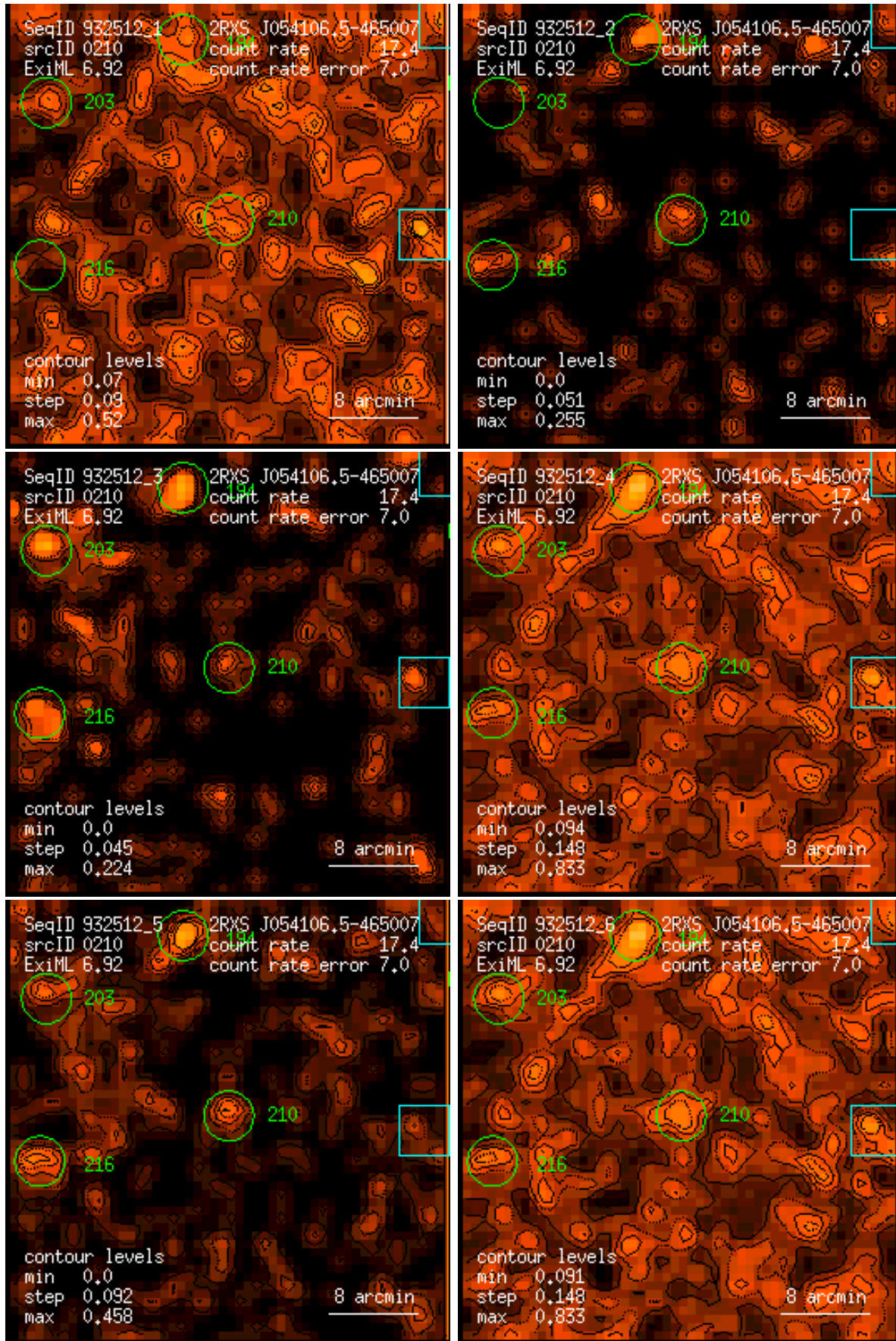
Figure 210: RASS 932512: detection 0210: band rate images, Gaussian filter: (1) PSPC channels 11 – 41, (2) 52 – 90, (3) 91 – 201, (4) 11 – 235, (5) 52 – 201, (6) 11 – 201. Broad band rates in counts/ks. Band rate contour levels in counts/ks/arcmin 2 .
