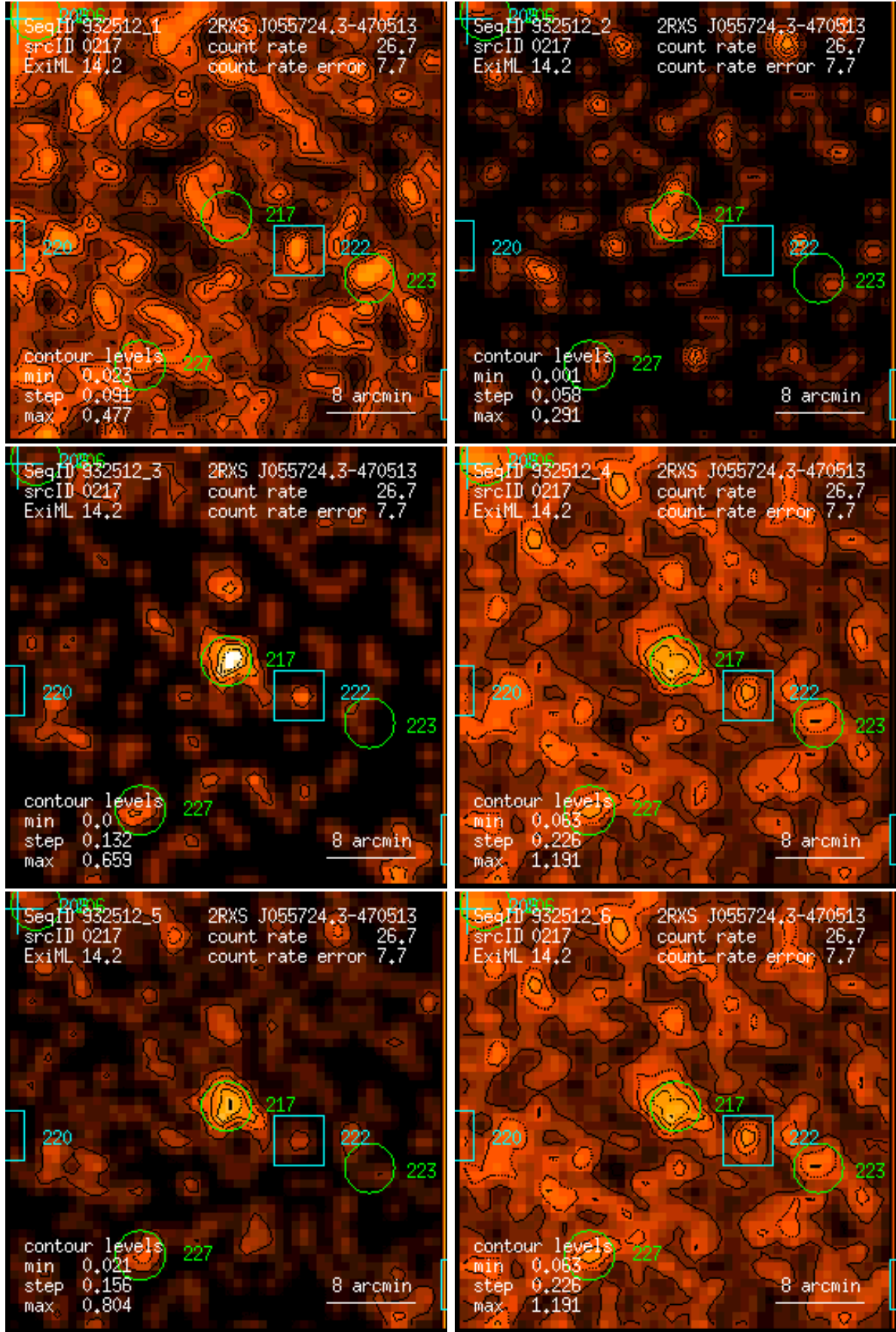
Figure 217: RASS 932512: detection 0217: band rate images, Gaussian filter: (1) PSPC channels 11 – 41, (2) 52 – 90, (3) 91 – 201, (4) 11 – 235, (5) 52 – 201, (6) 11 – 201. Broad band rates in counts/ks. Band rate contour levels in counts/ks/arcmin 2 .
