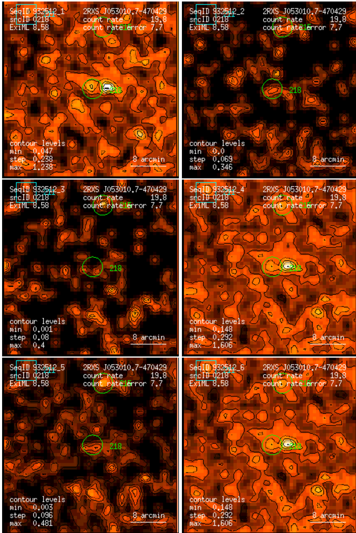
Figure 218: RASS 932512: detection 0218: band rate images, Gaussian filter: (1) PSPC channels 11 – 41, (2) 52 – 90, (3) 91 – 201, (4) 11 – 235, (5) 52 – 201, (6) 11 – 201. Broad band rates in counts/ks. Band rate contour levels in counts/ks/arcmin 2 .
