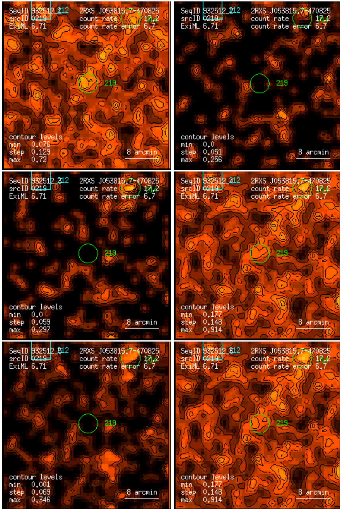
Figure 219: RASS 932512: detection 0219: band rate images, Gaussian filter: (1) PSPC channels 11 – 41, (2) 52 – 90, (3) 91 – 201, (4) 11 – 235, (5) 52 – 201, (6) 11 – 201. Broad band rates in counts/ks. Band rate contour levels in counts/ks/arcmin 2 .
