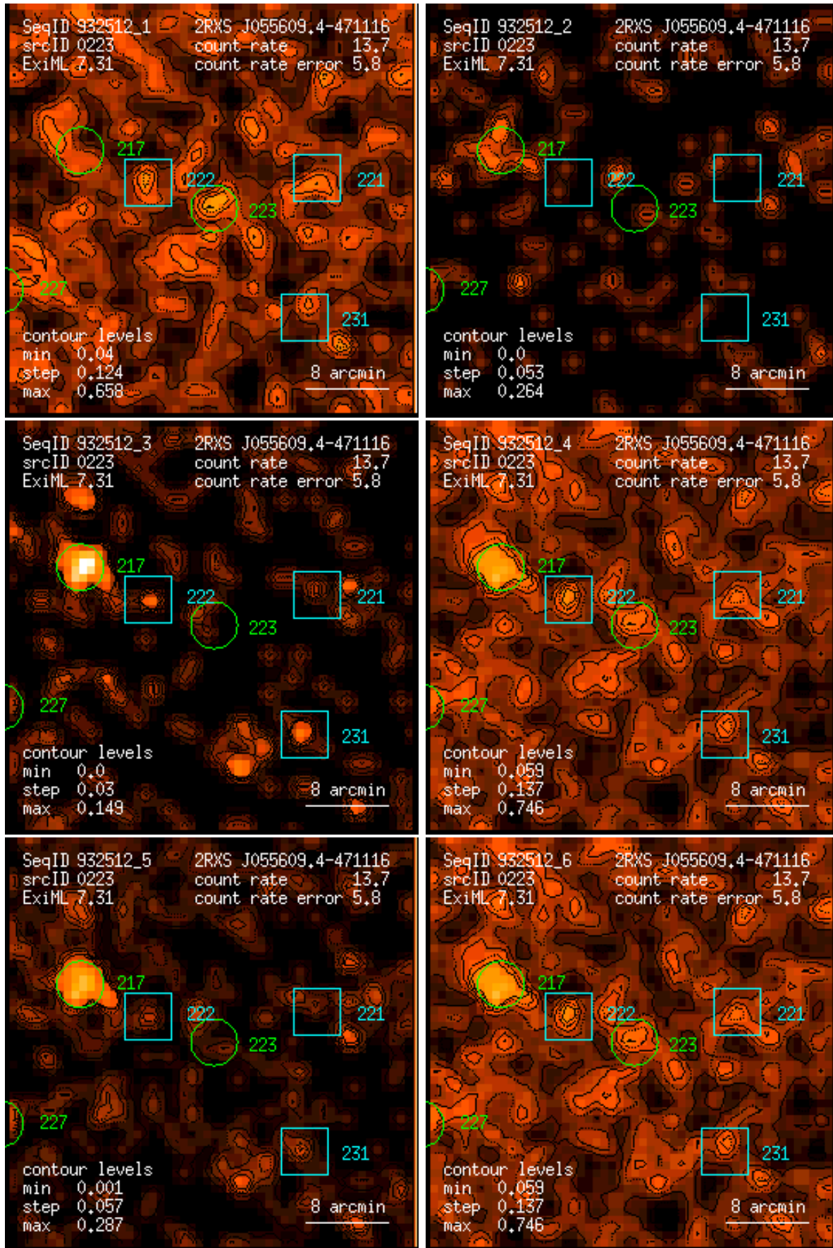
Figure 223: RASS 932512: detection 0223: band rate images, Gaussian filter: (1) PSPC channels 11 – 41, (2) 52 – 90, (3) 91 – 201, (4) 11 – 235, (5) 52 – 201, (6) 11 – 201. Broad band rates in counts/ks. Band rate contour levels in counts/ks/arcmin 2 .
